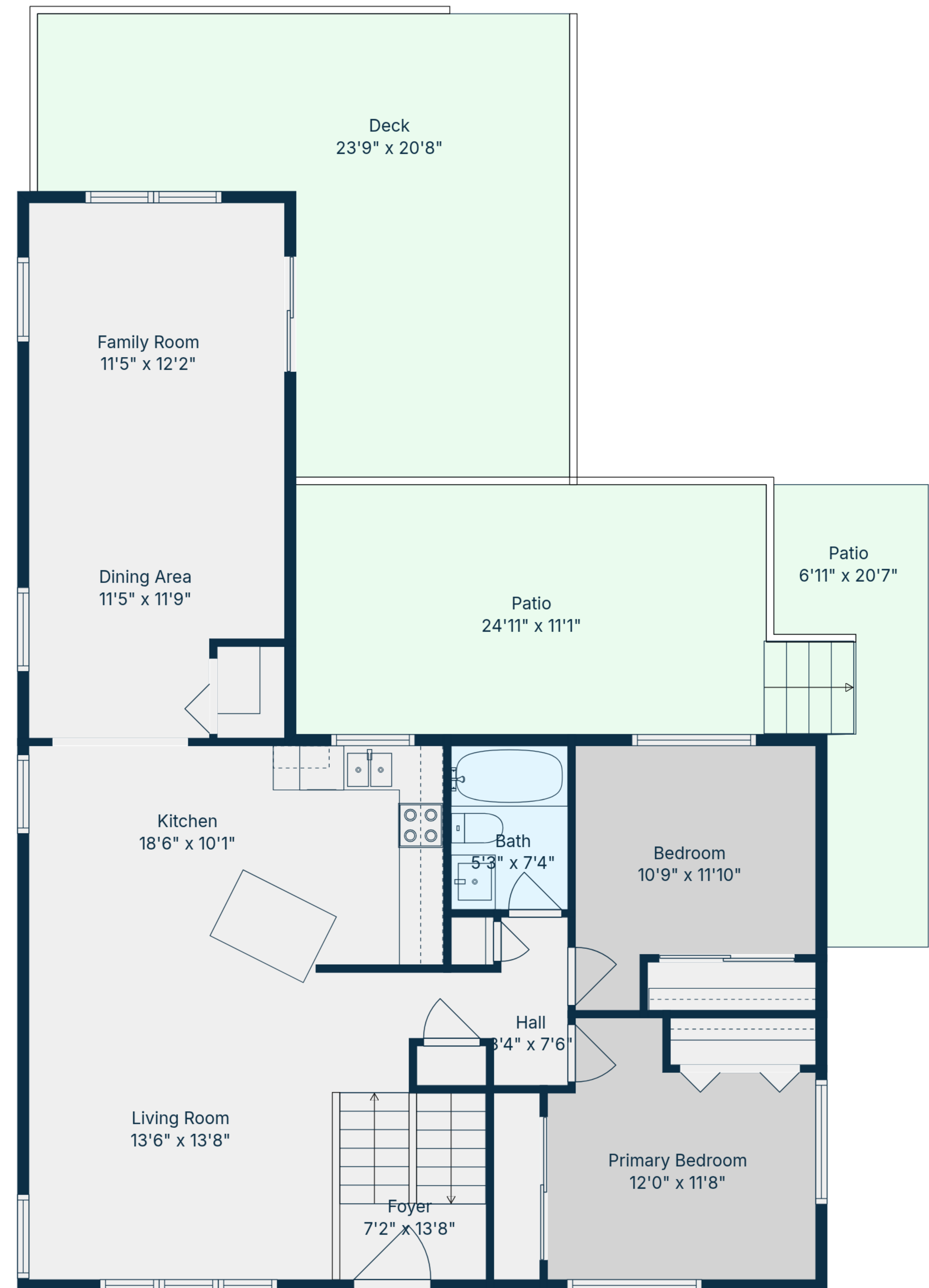
1st Floor
