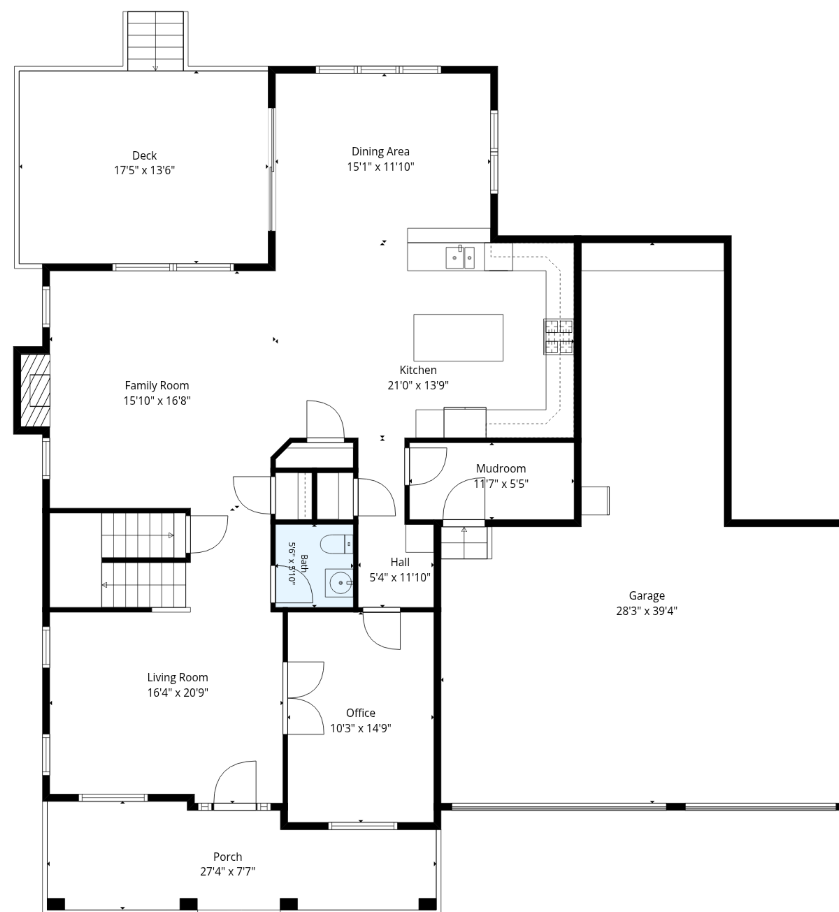
1st Floor
