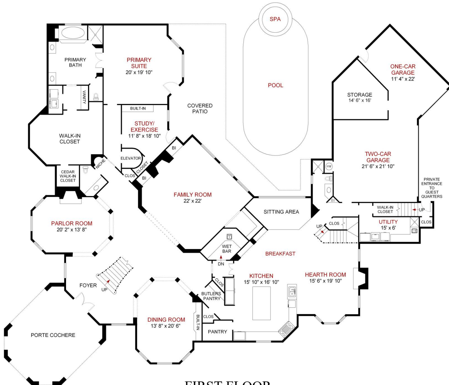
FIRST FLOOR
