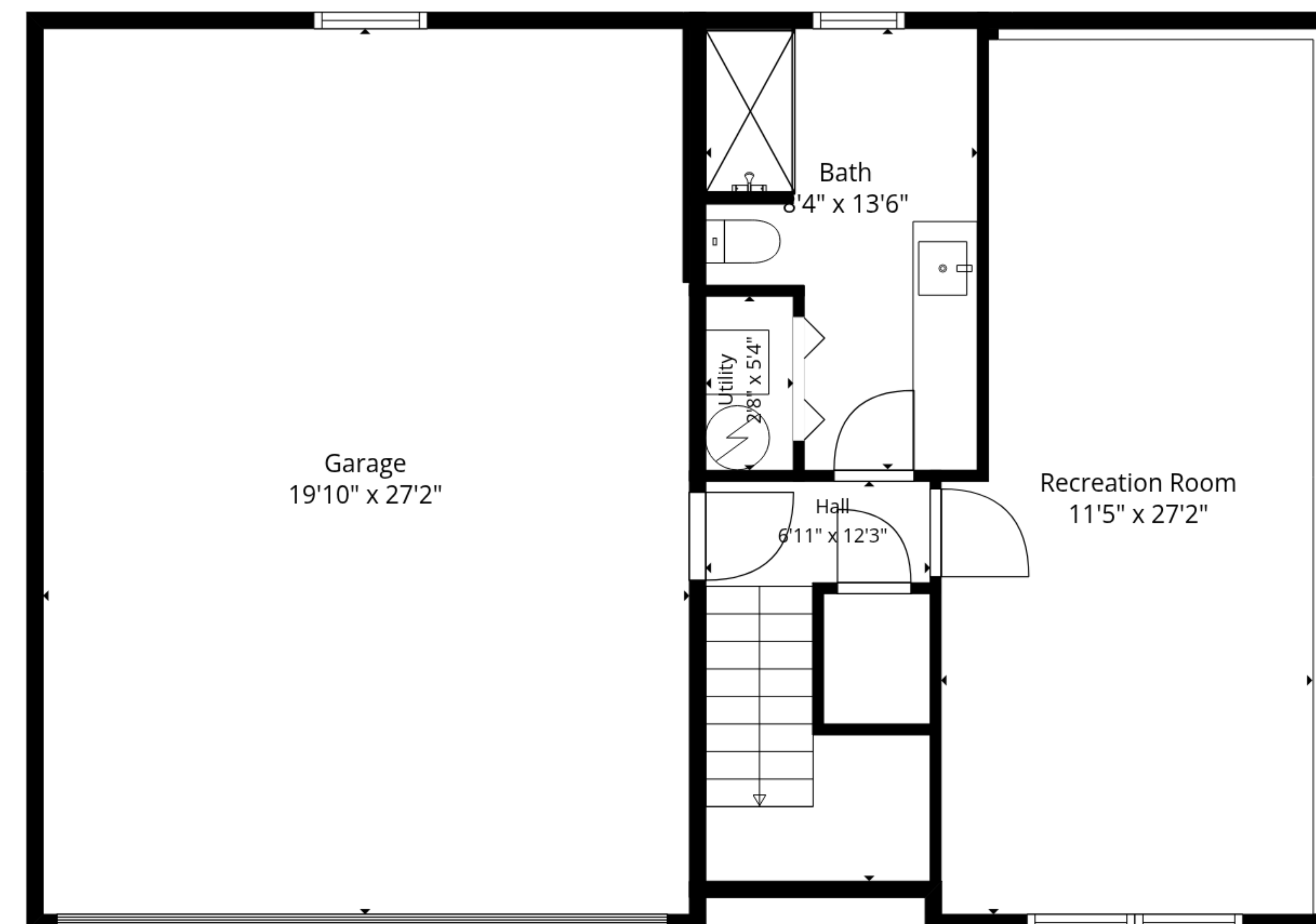
2nd Floor
