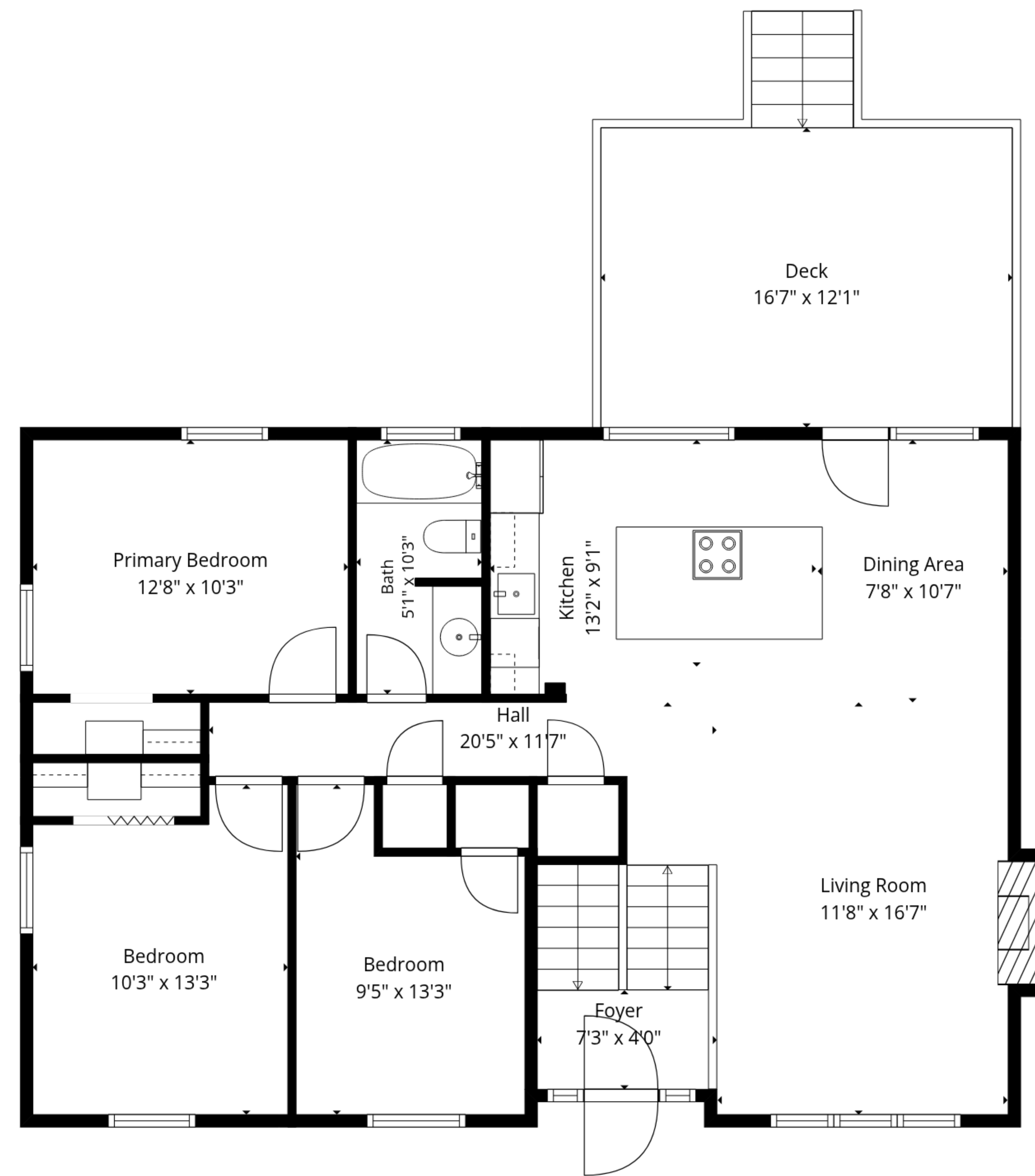
2nd Floor
