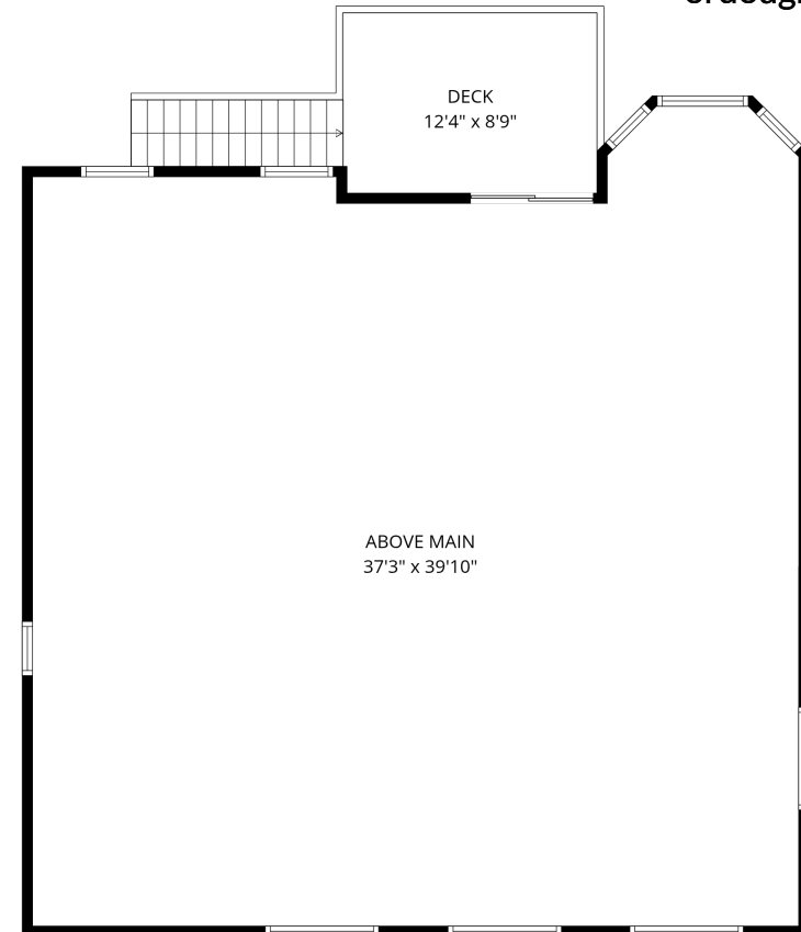
FLOOR 2
