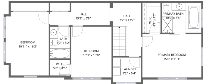
2nd floor
