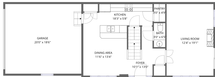
1st floor
