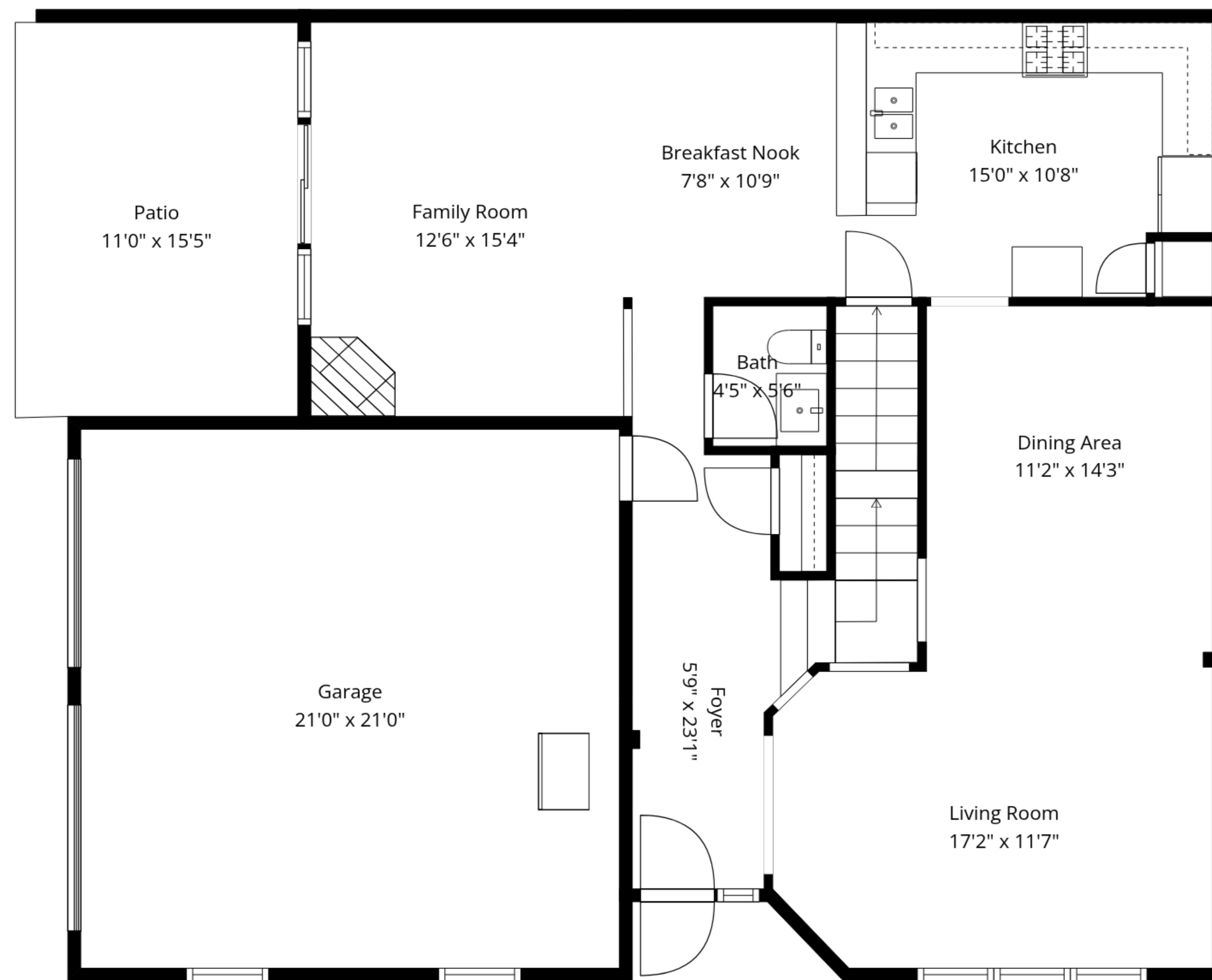
1st Floor
