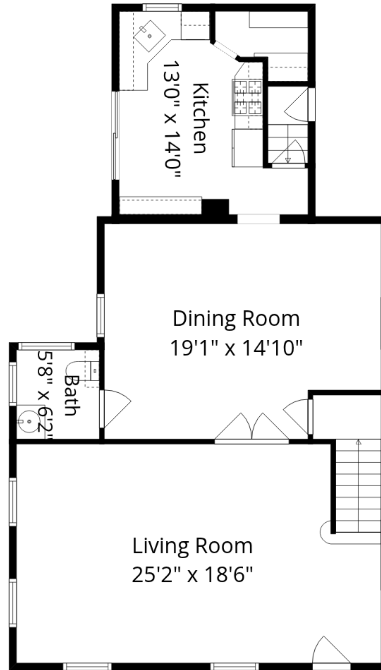
Main Floor
