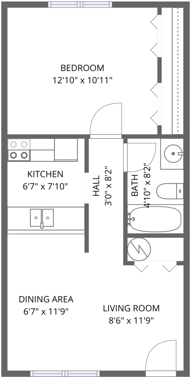
FLOOR 1
