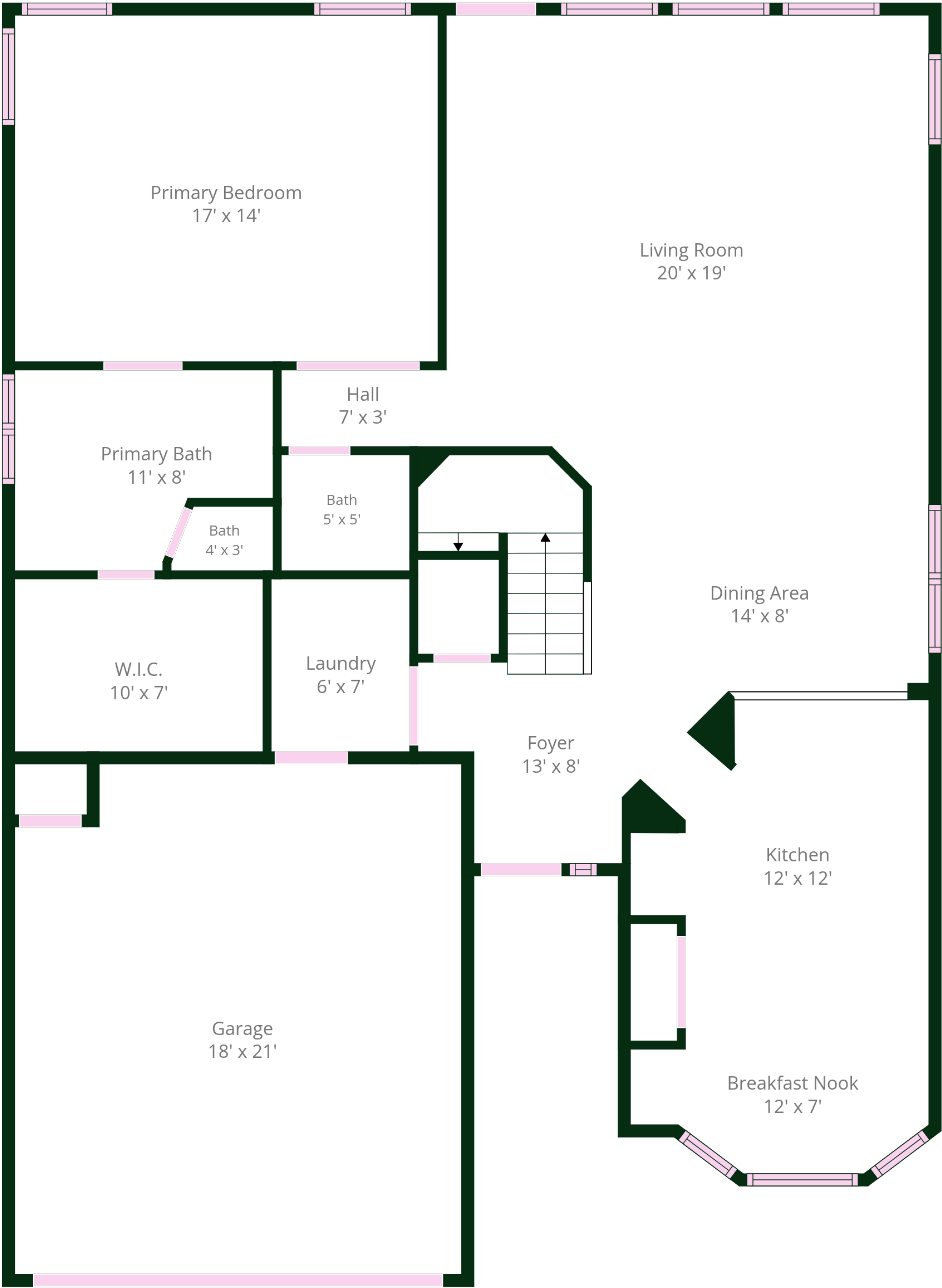
1st Floor
