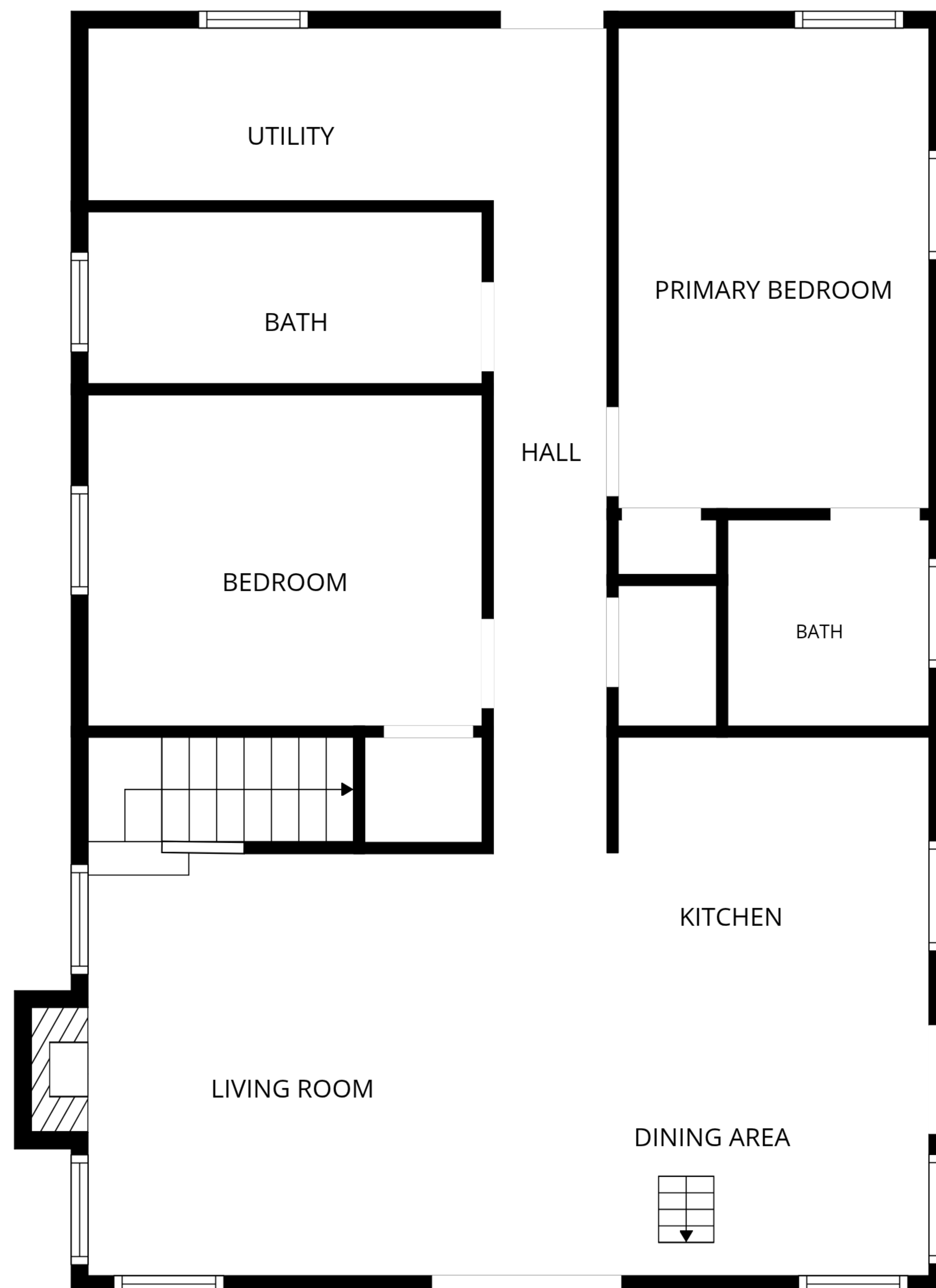
1st floor
