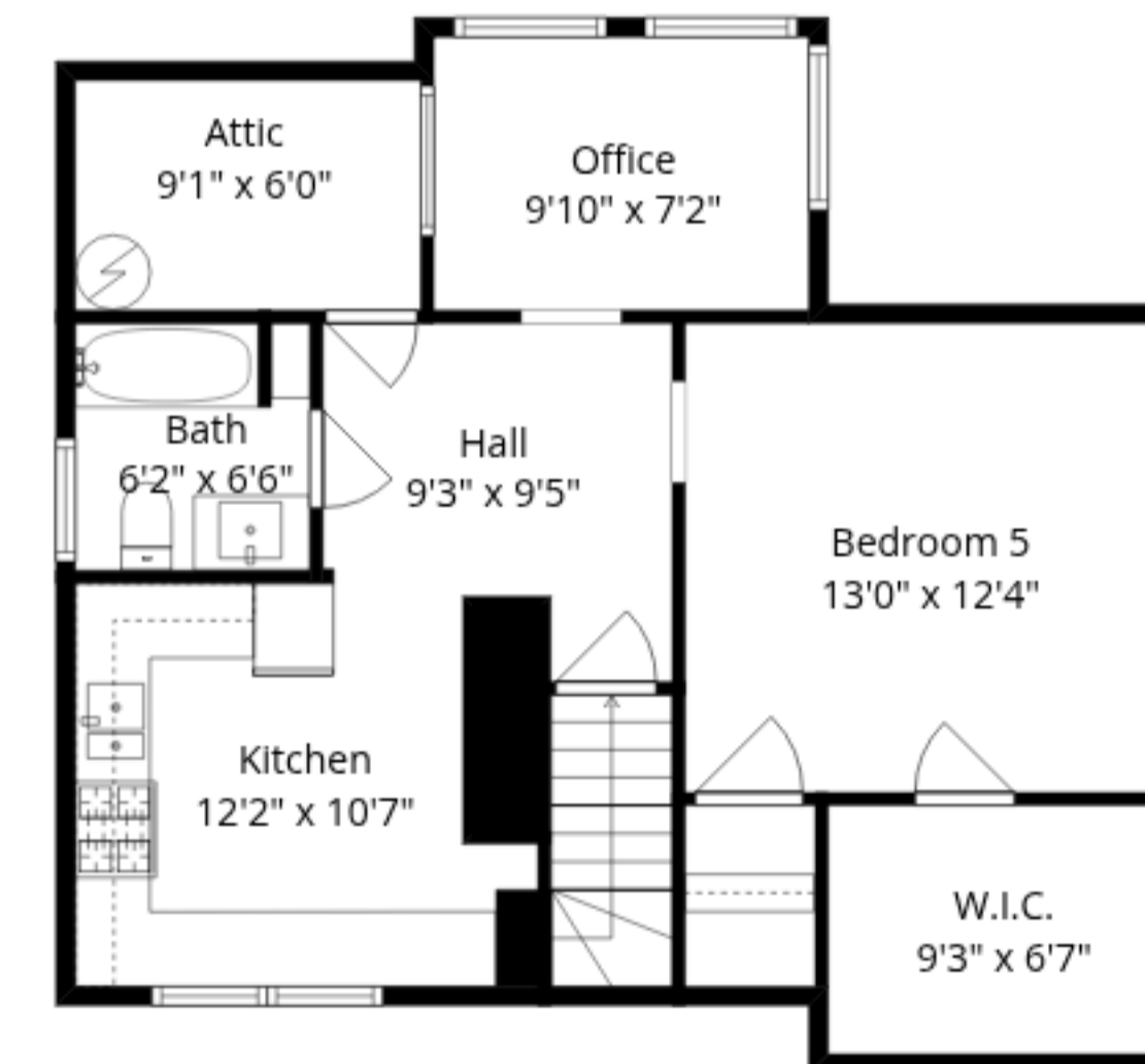
3rd Floor
