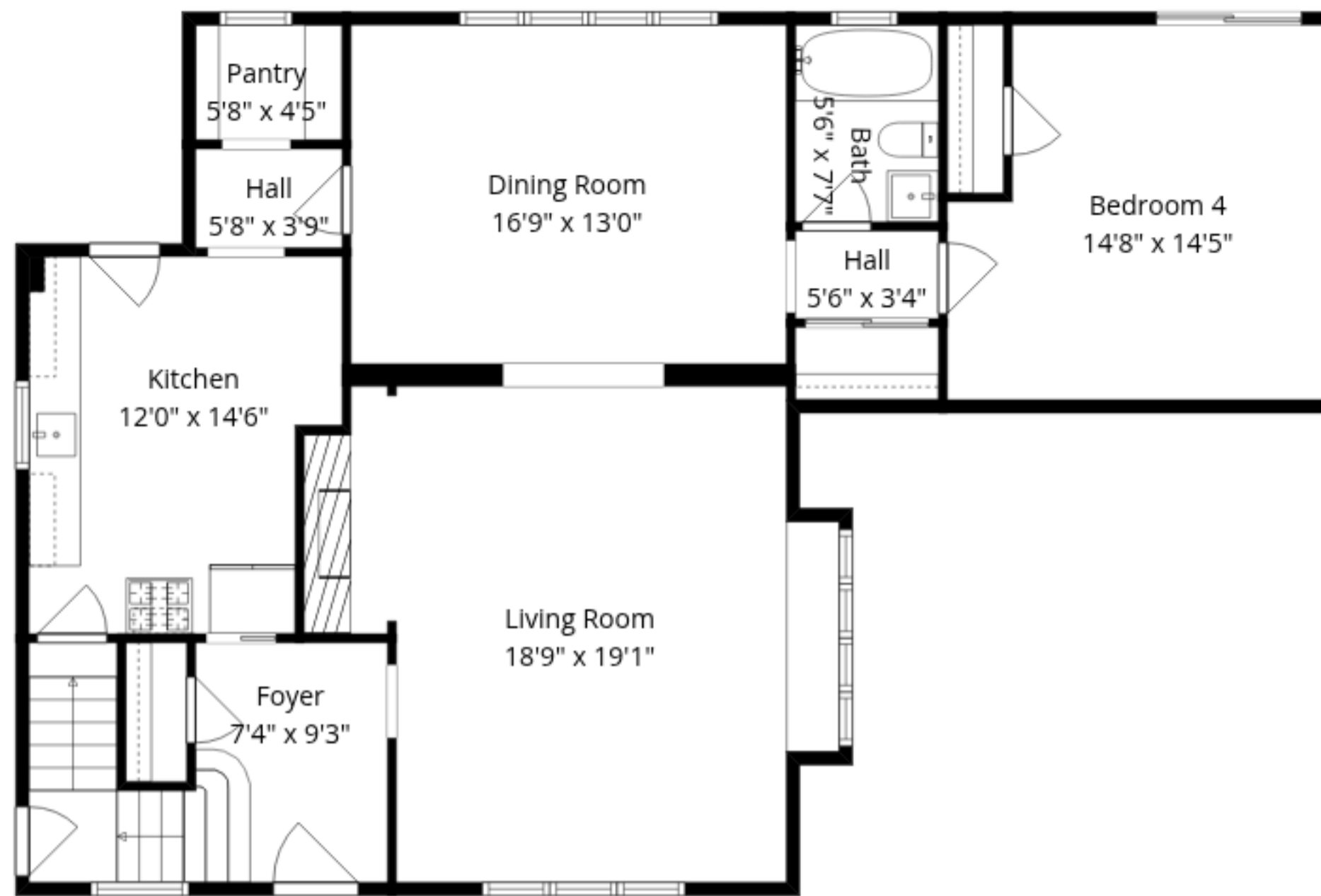
Main Floor
