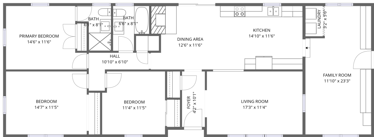
FLOOR 1
