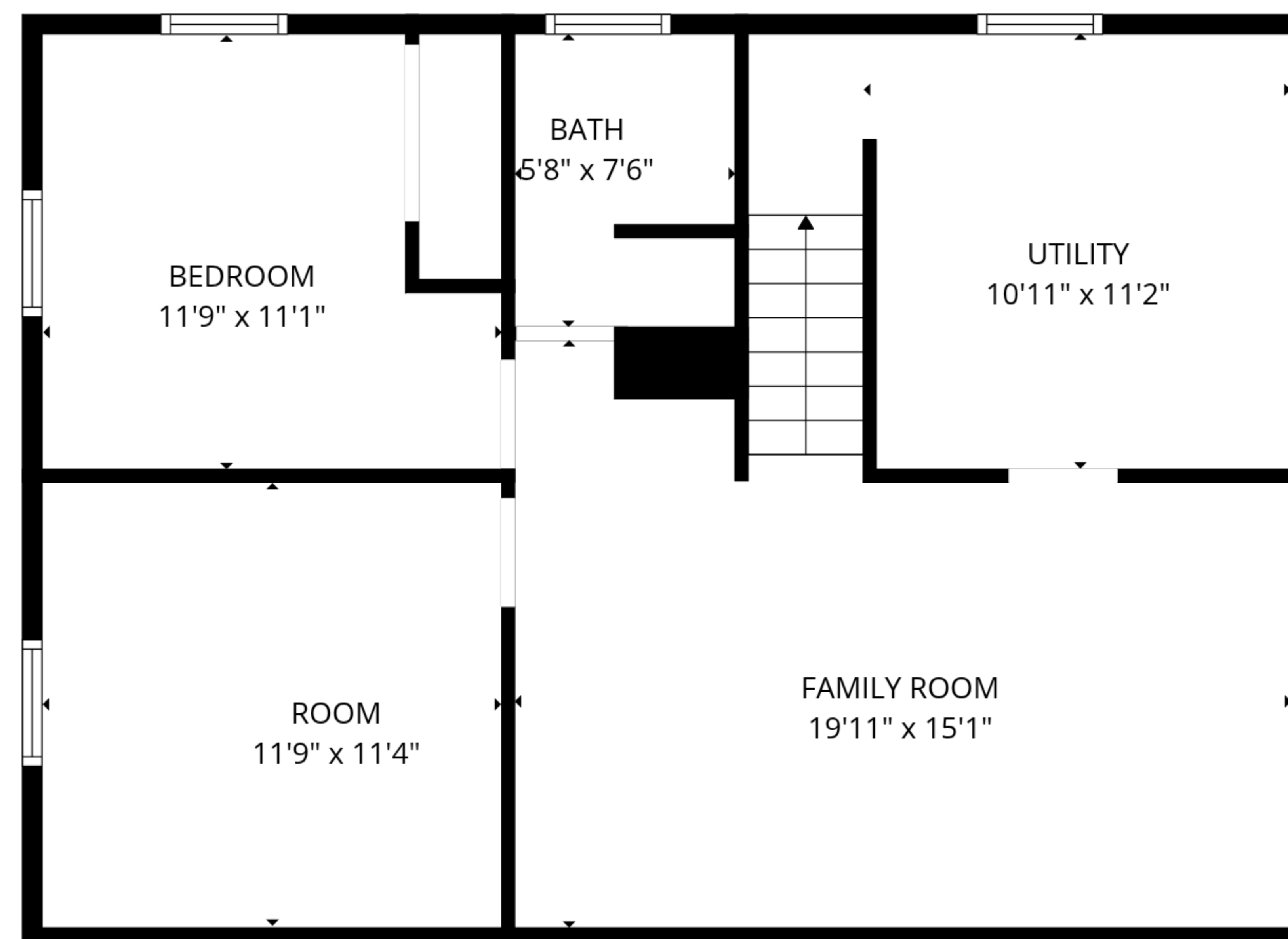
1st floor
