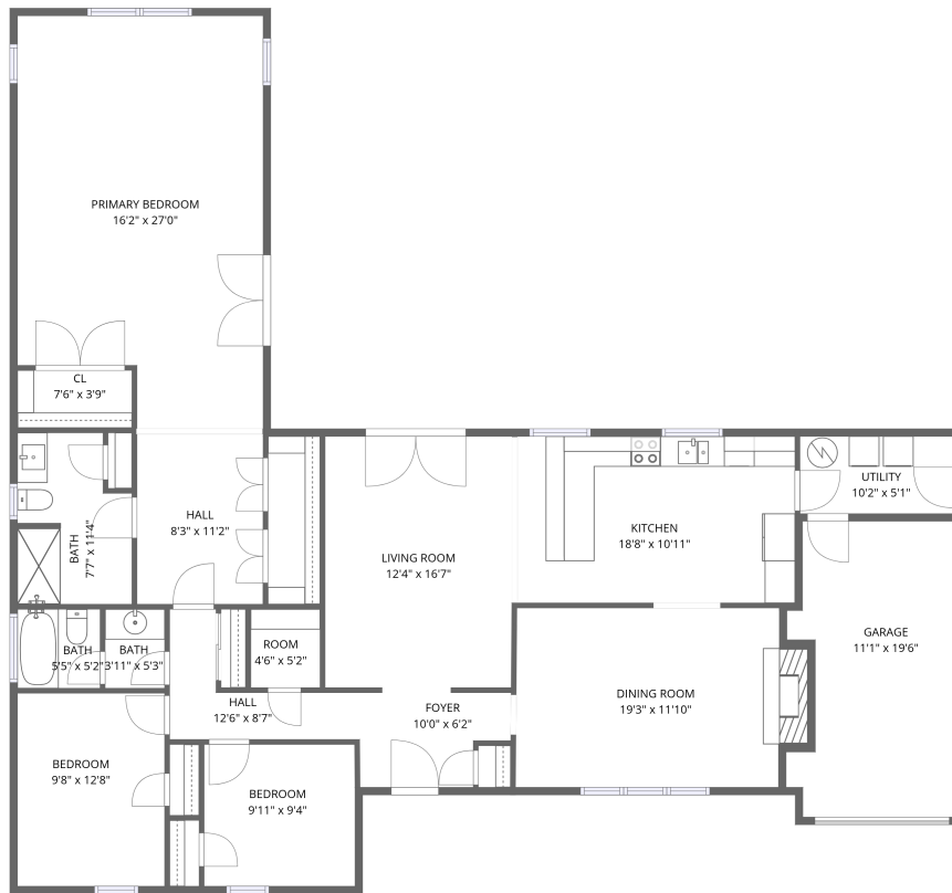
1st floor
