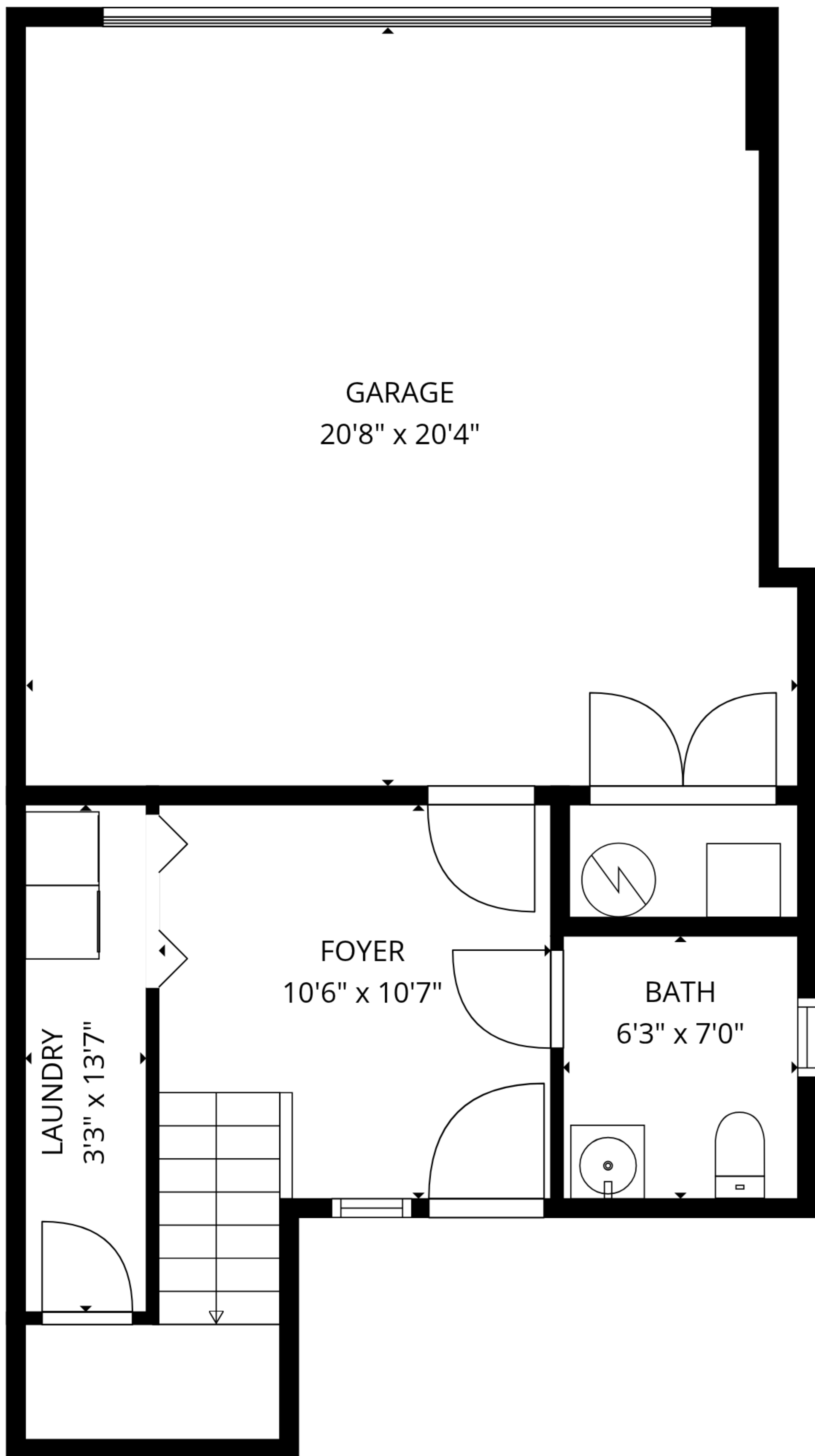
1st floor
