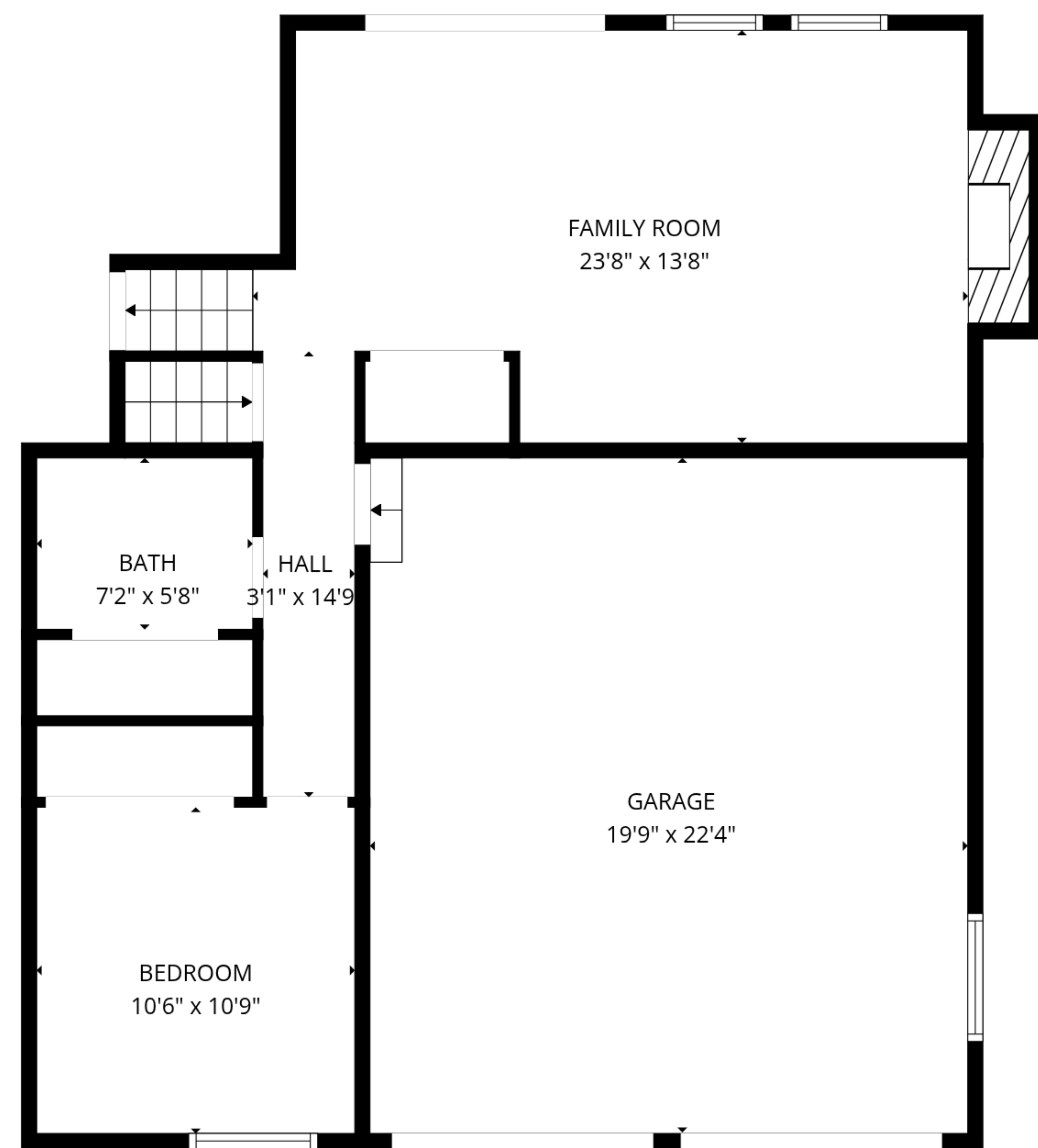
1st floor
