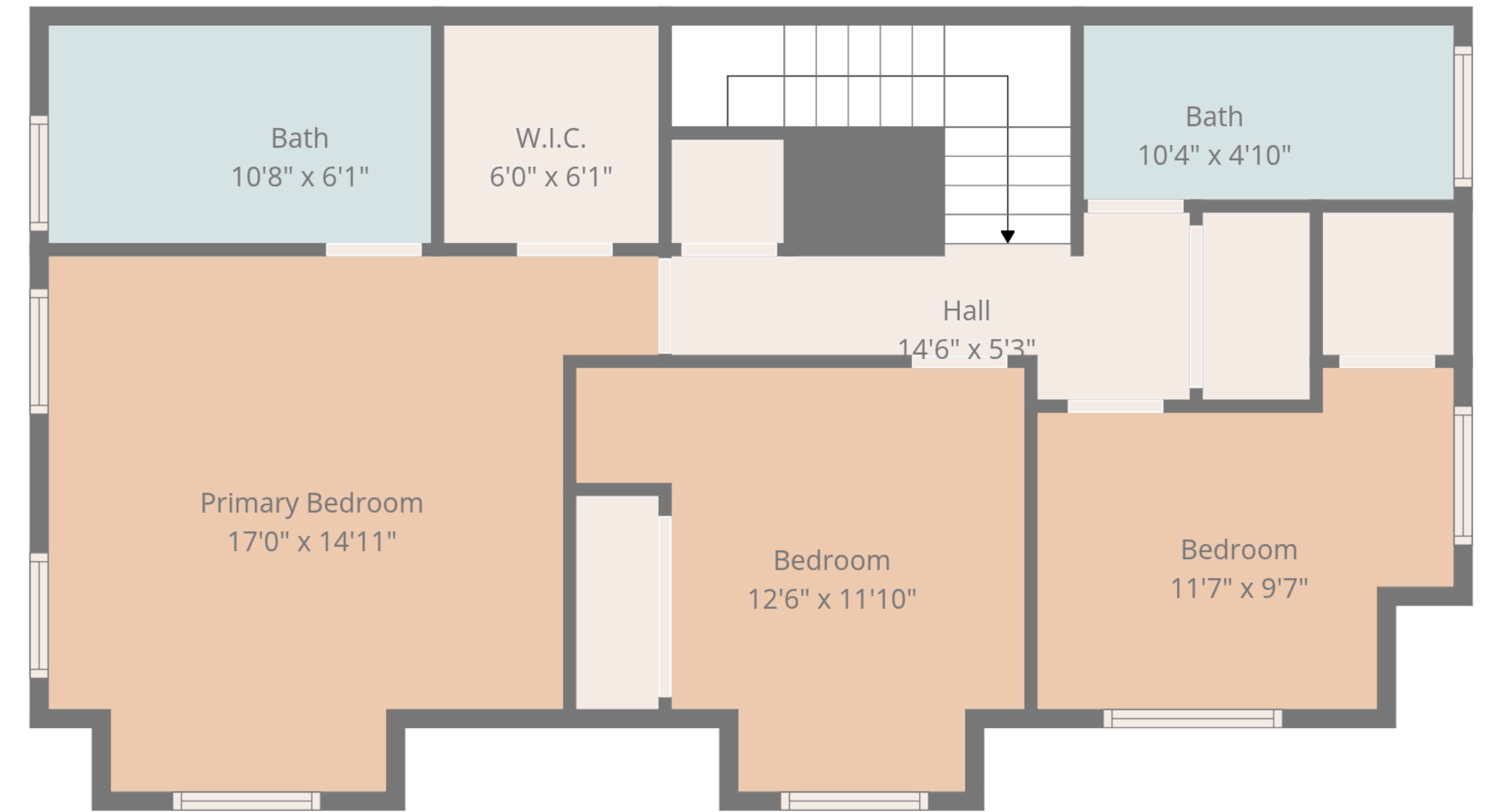
2nd Floor
