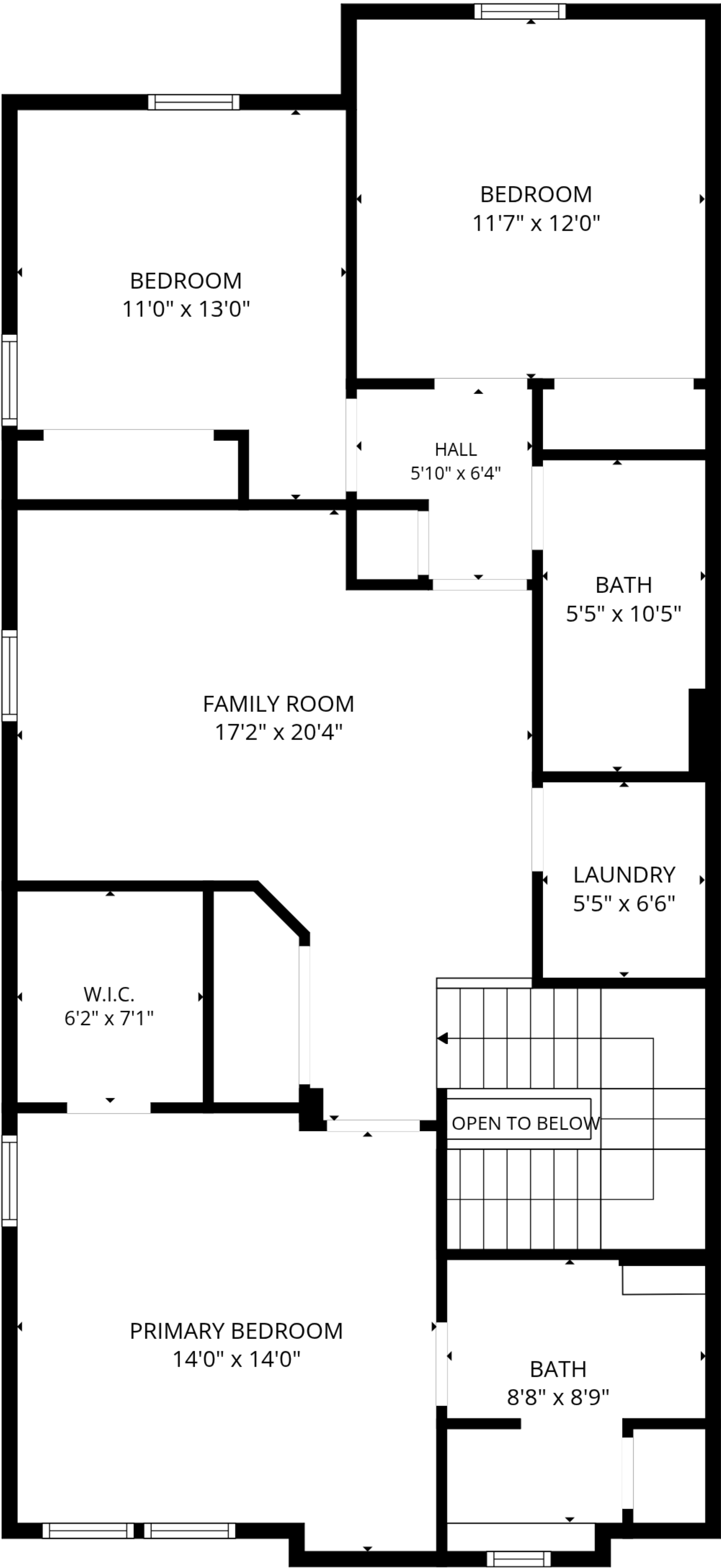
2nd floor
