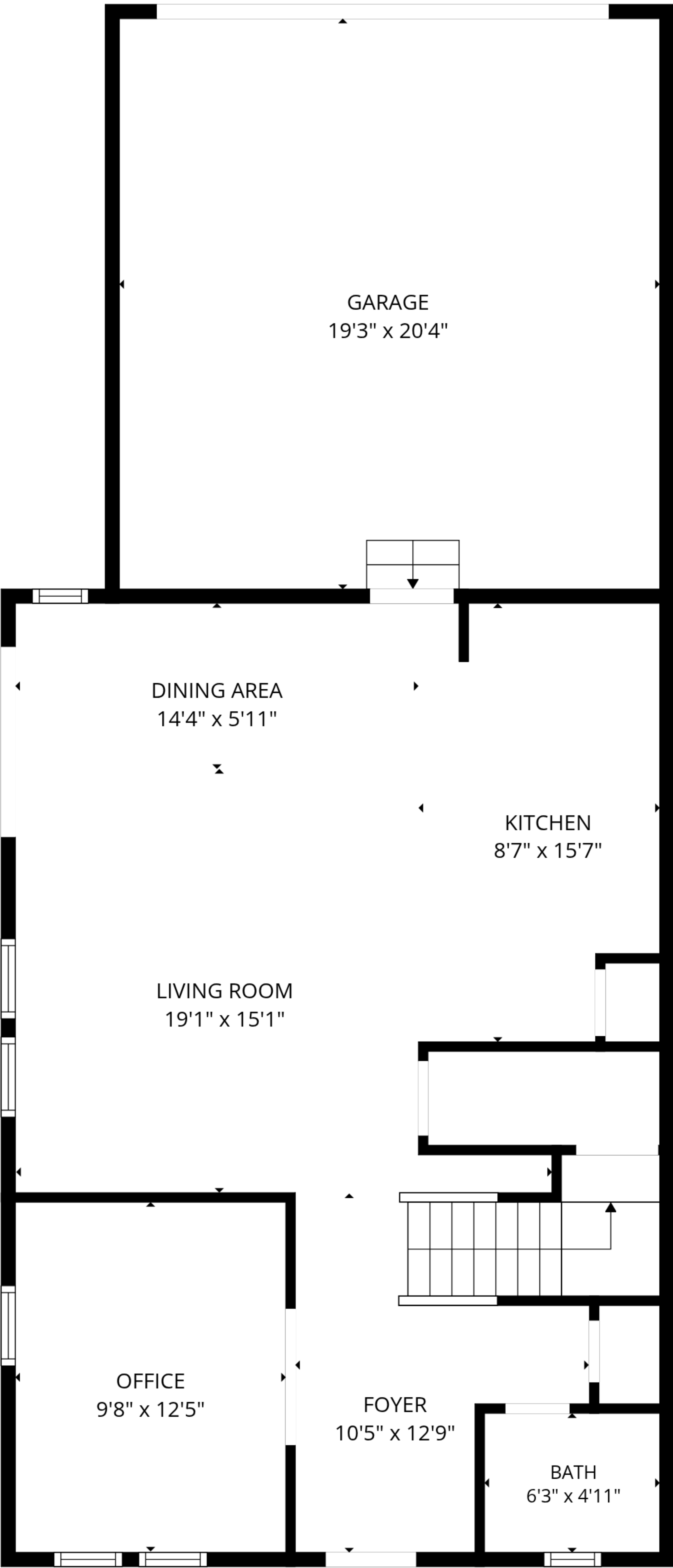
1st floor
