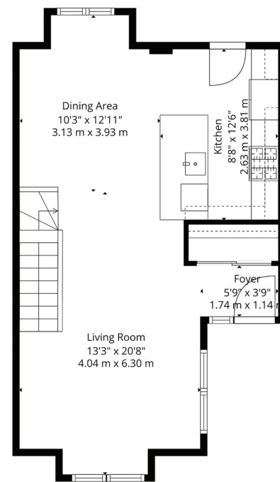
TOTAL: 2076 sq. ft., 193 m 2 Basement: 491 sq. ft., 46 m 2 , 1st floor: 525 sq. ft., 49 m 2 , 2nd floor: 540 sq. ft., 50 m 2 , 3rd floor: 520 sq. ft., 48 m 2 EXCLUDED AREAS: UTILITY: 29 sq. ft., 3 m 2 , WALLS: 205 sq. ft., 18 m 2
