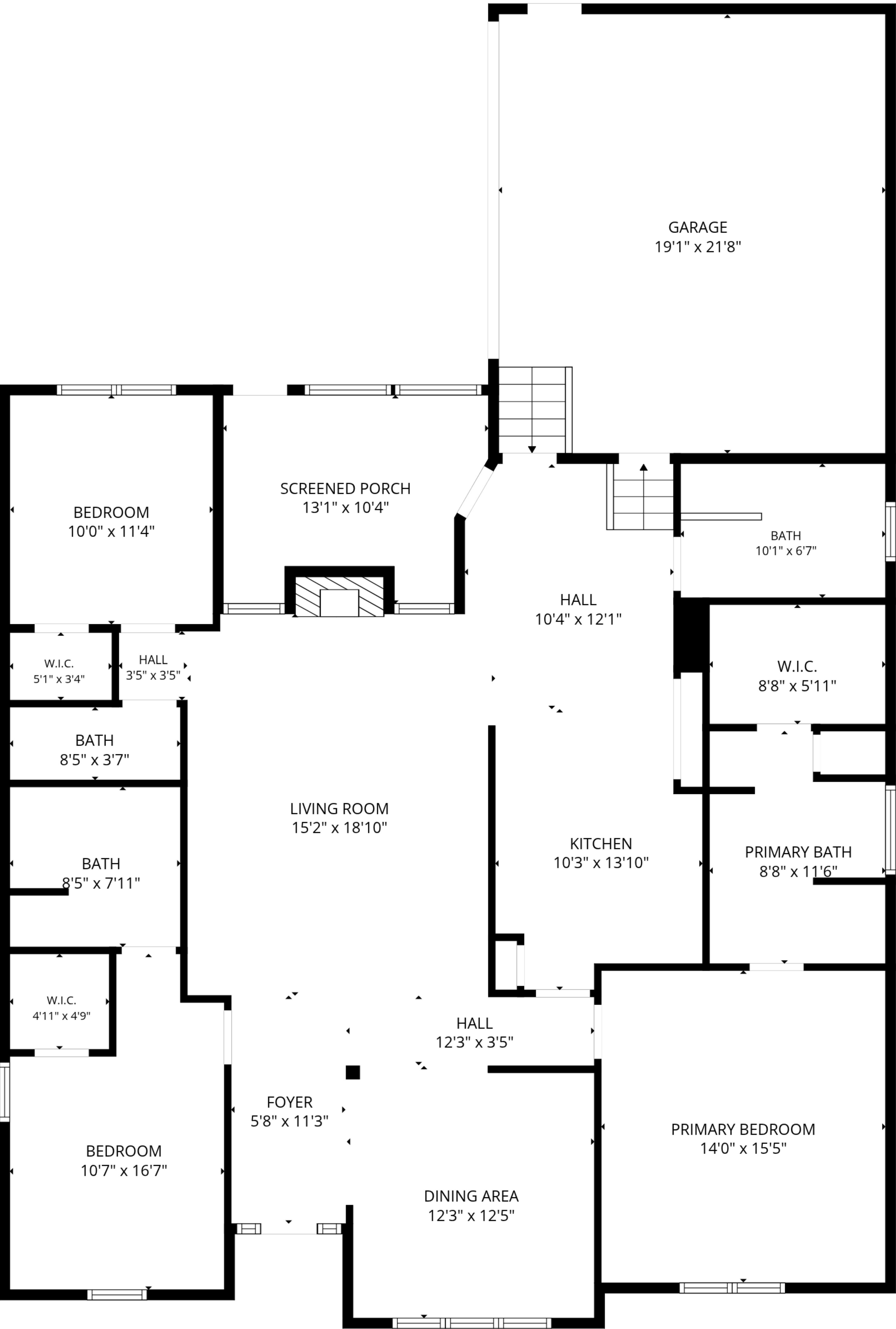
1st floor
