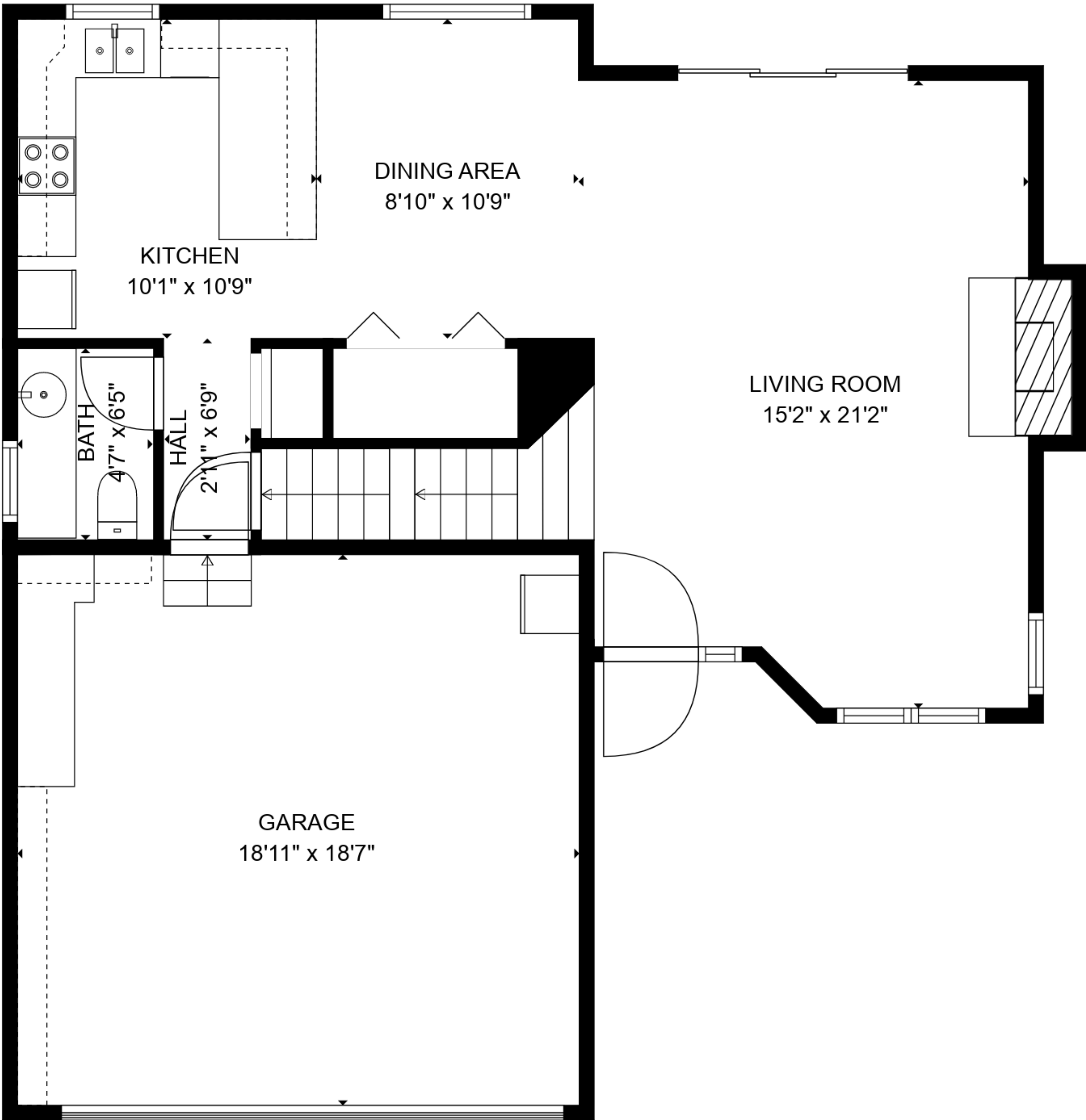
FLOOR 2
