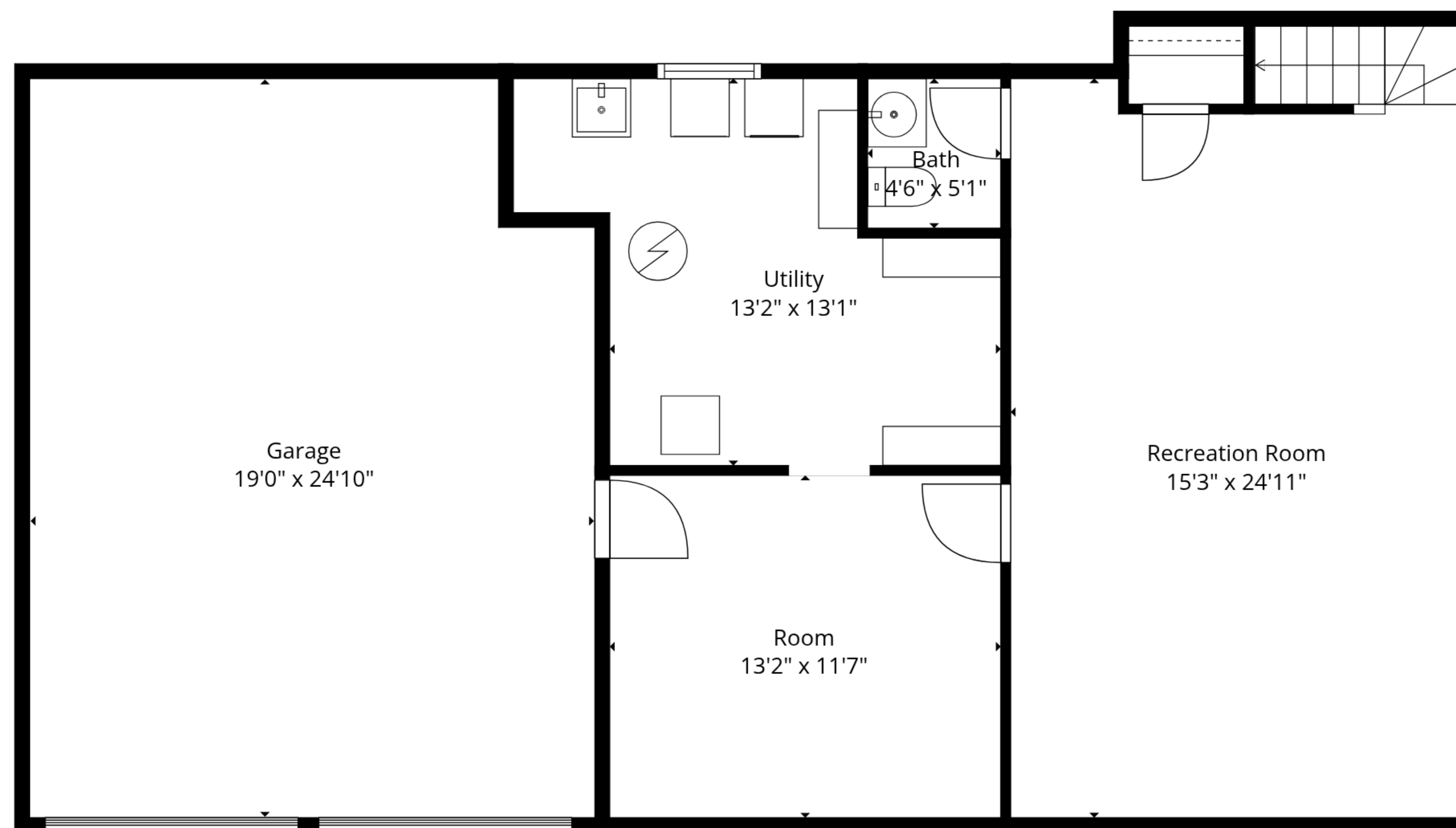
1st Floor
