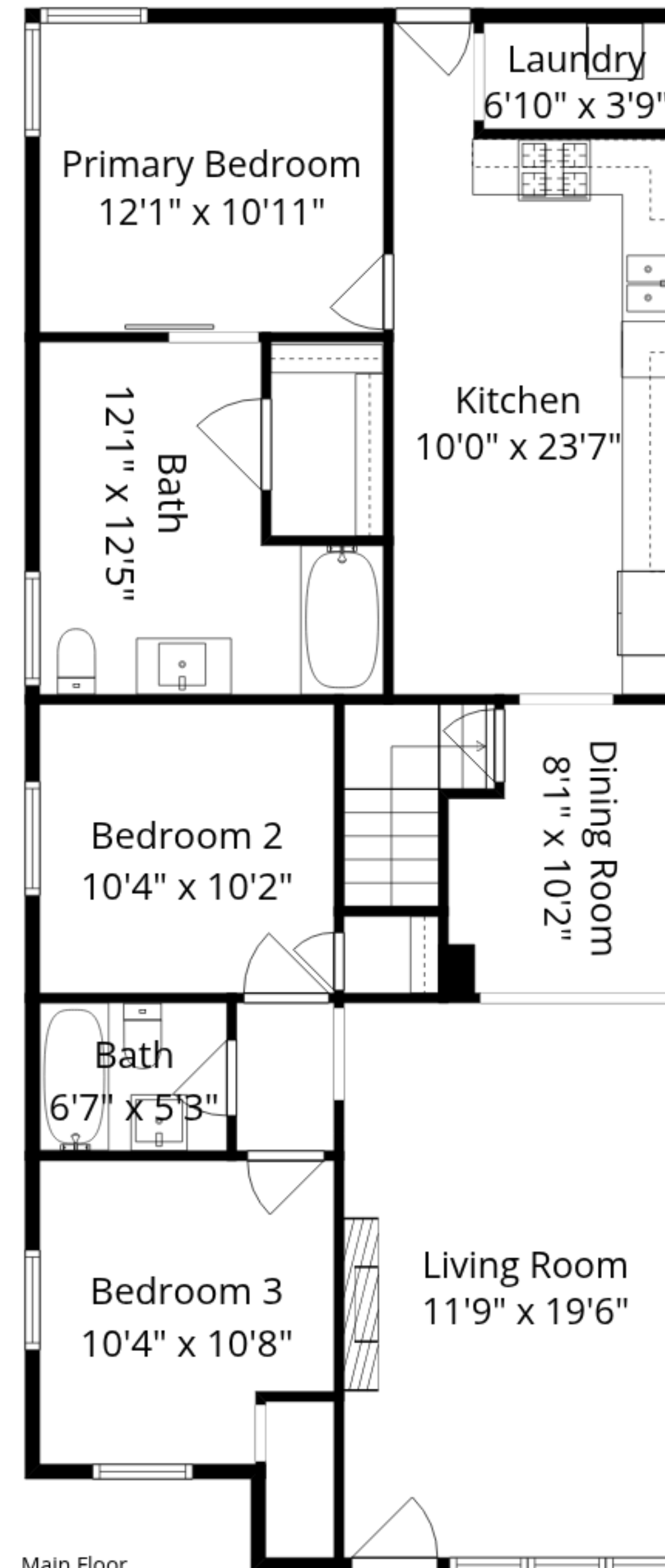
Main Floor
