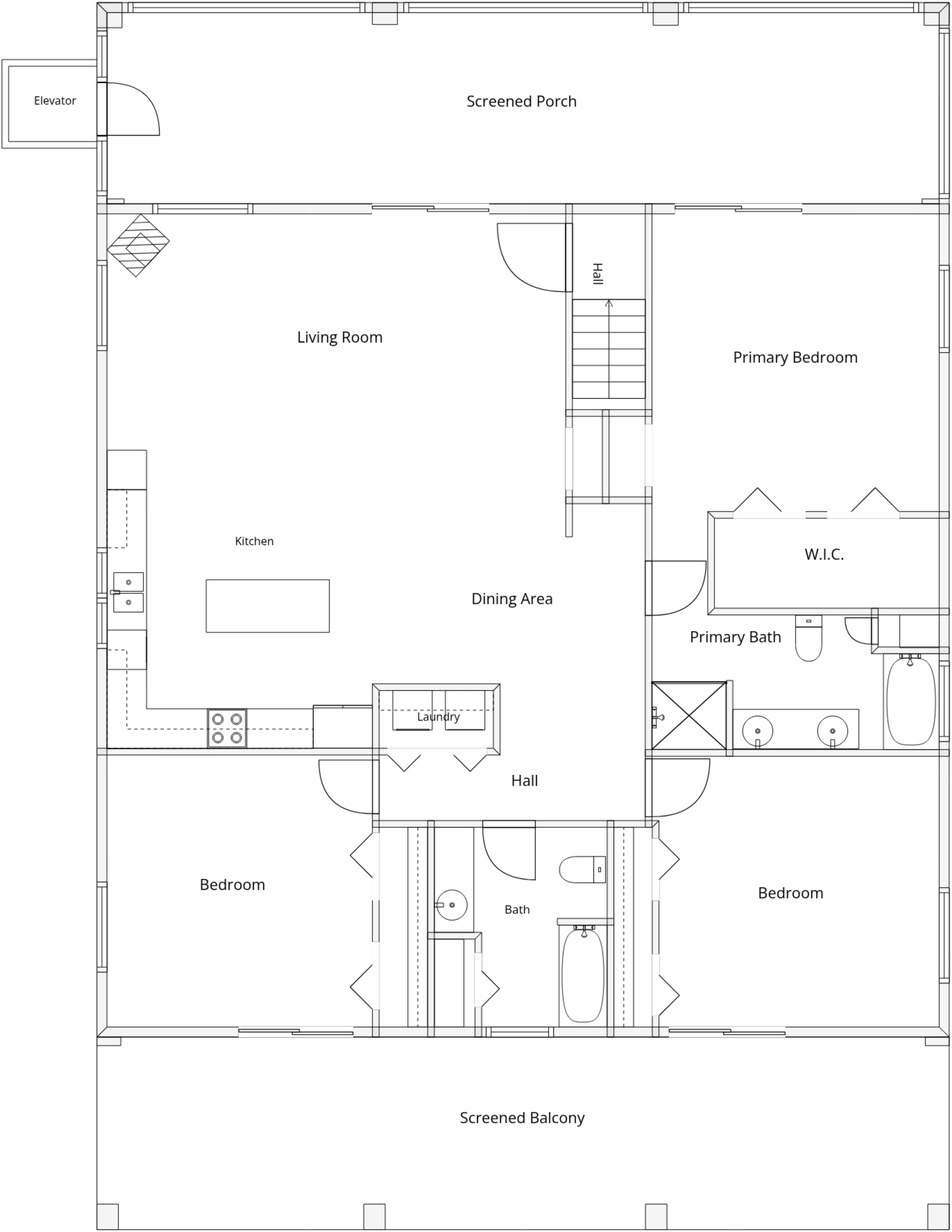
2nd Floor
