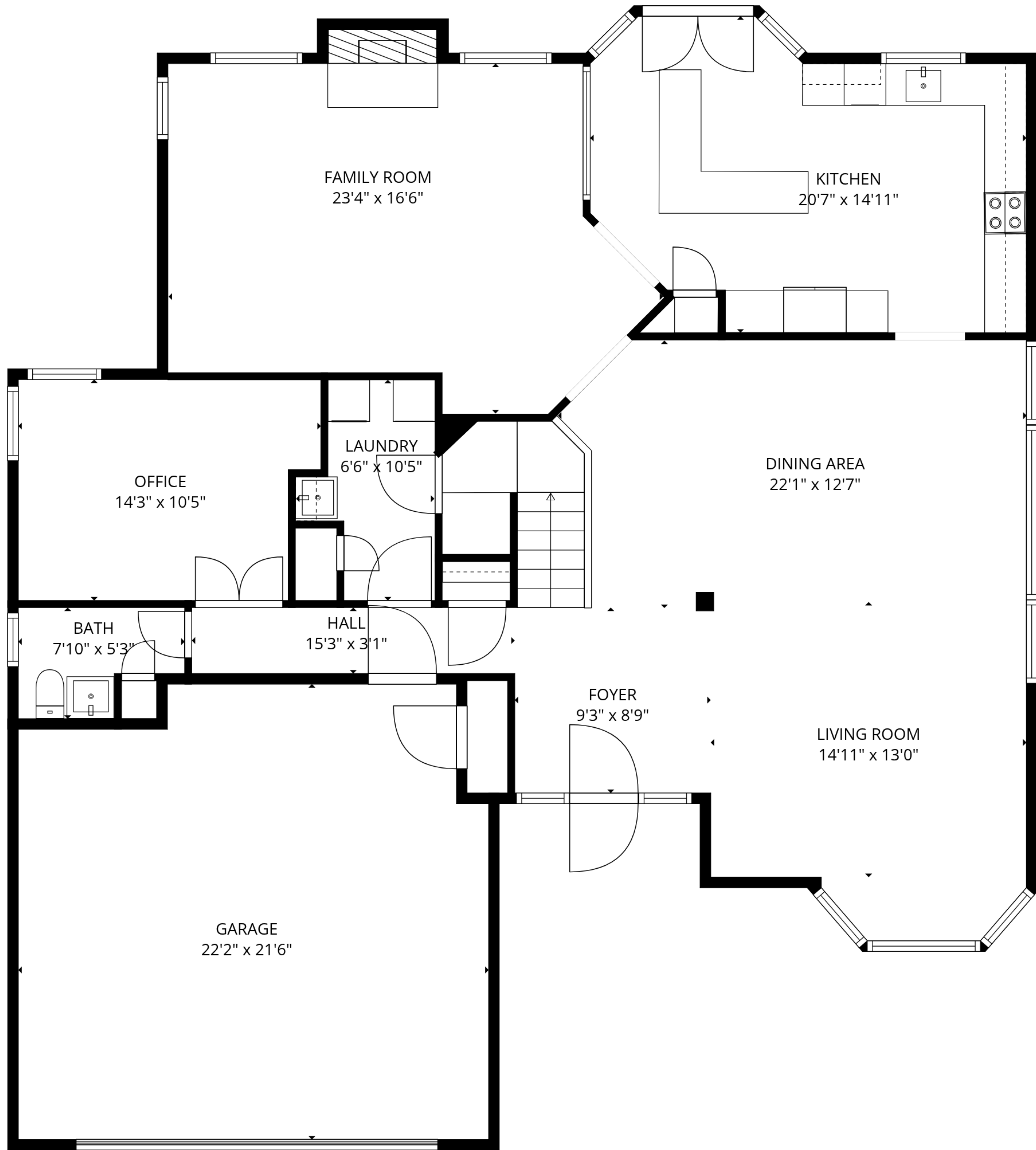
FLOOR 1
