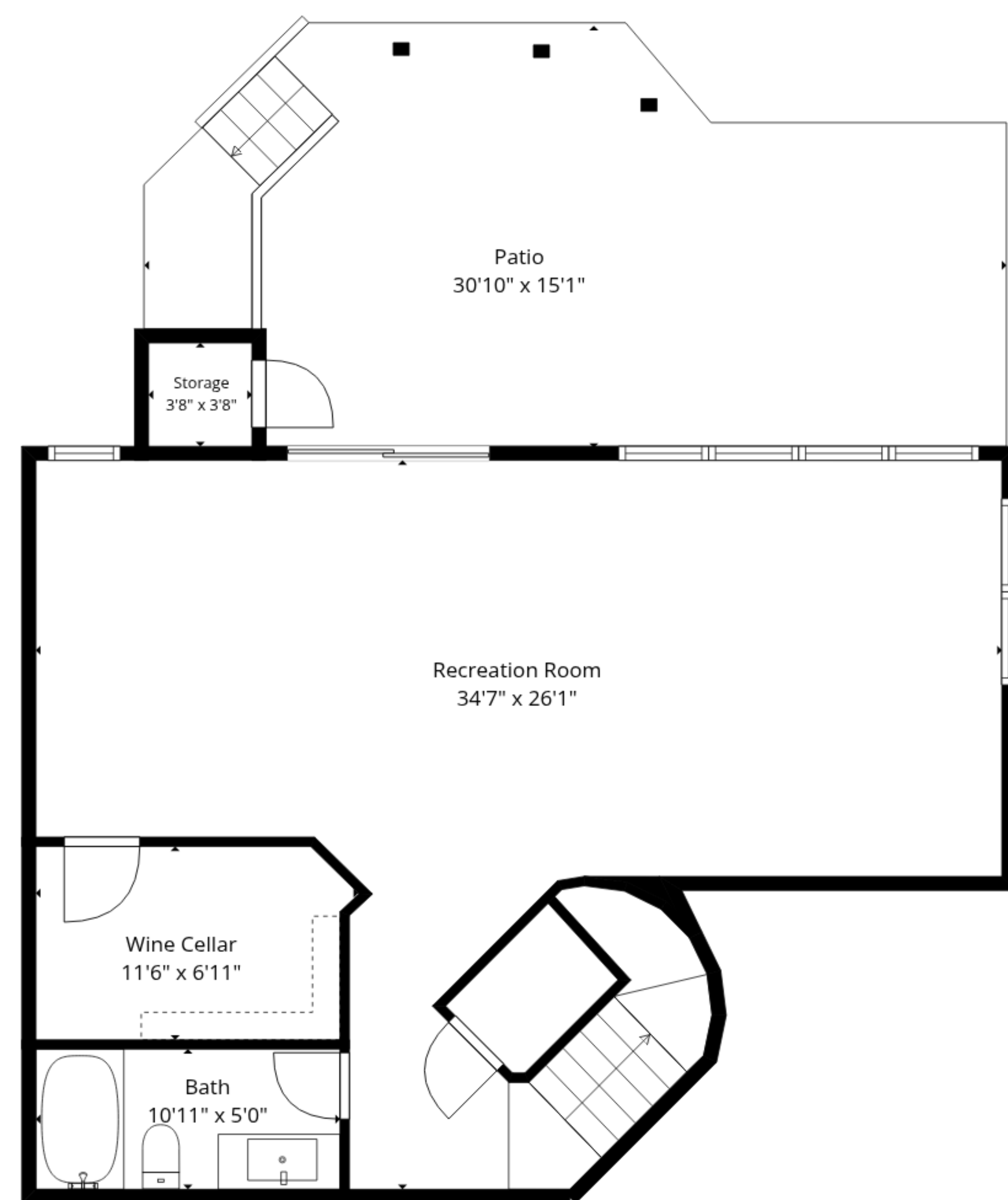
Lower Level
