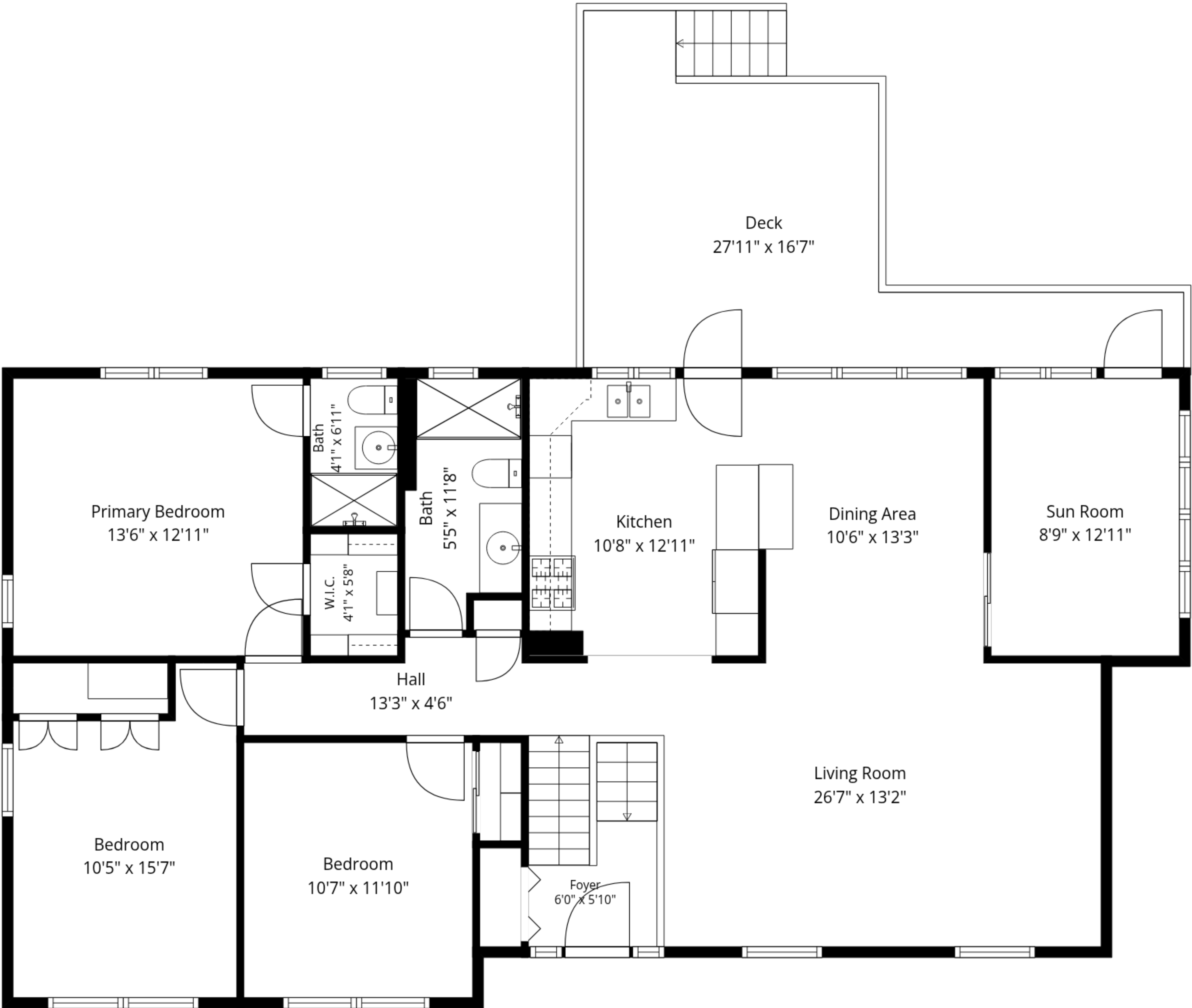
1st Floor
