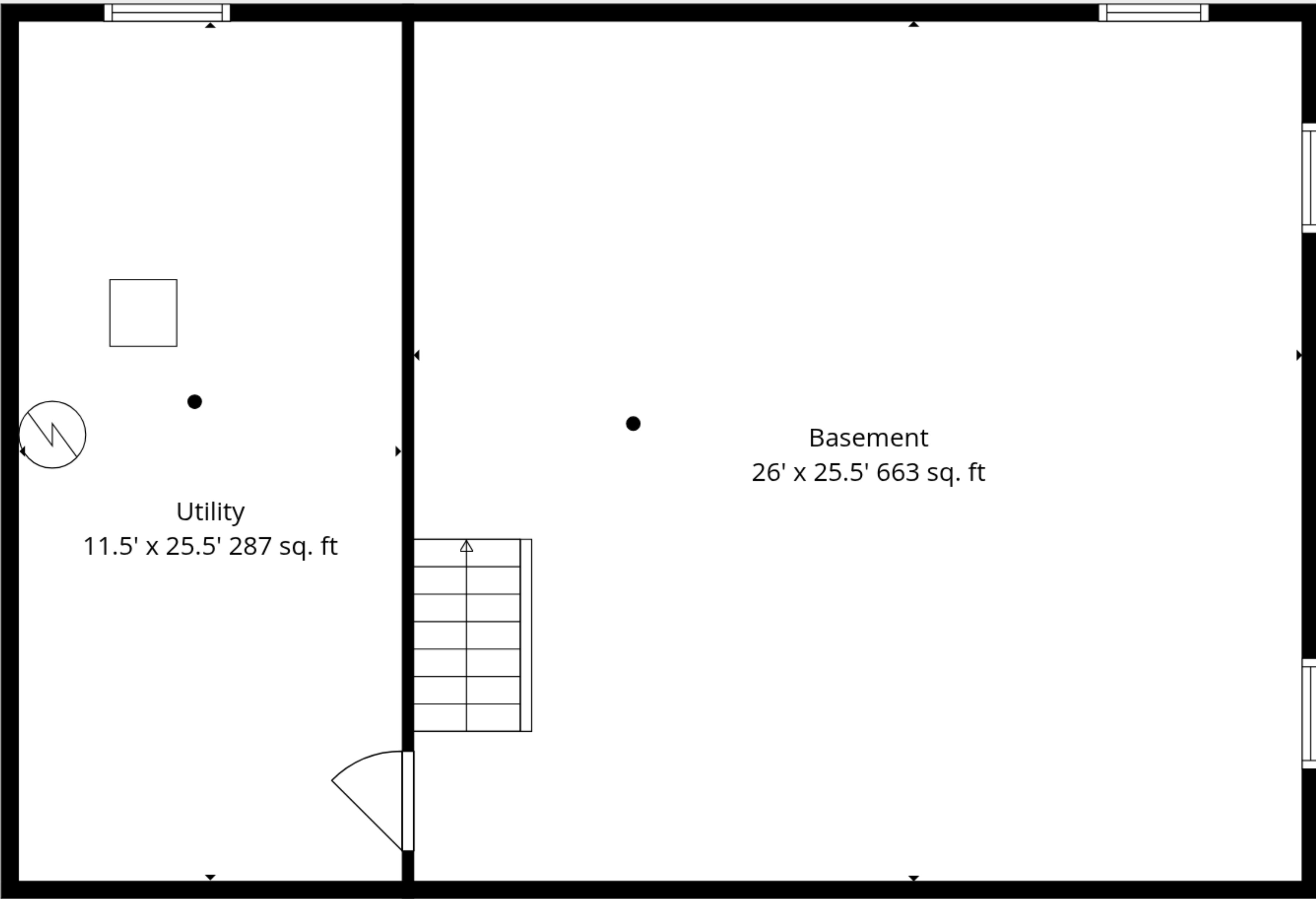
Basement
