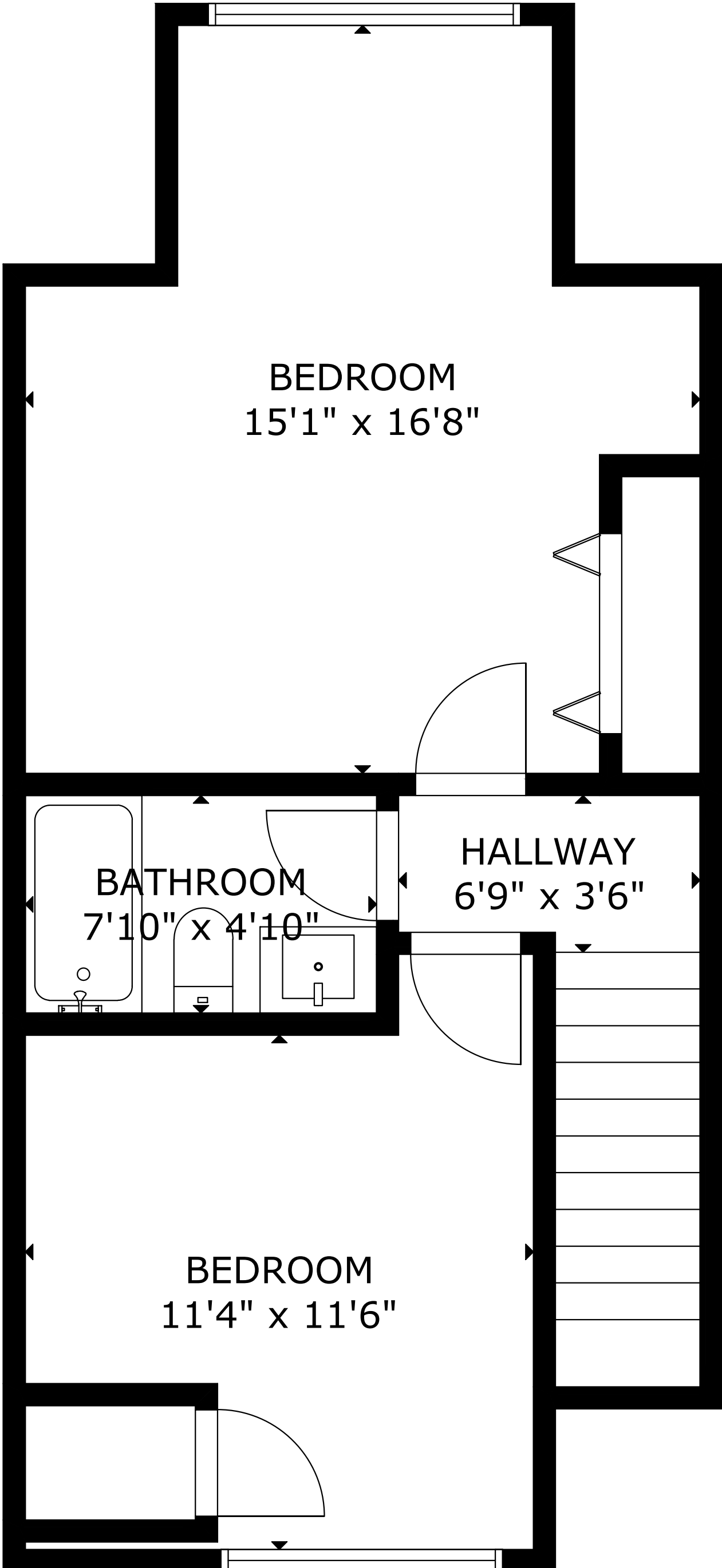
FLOOR 2
