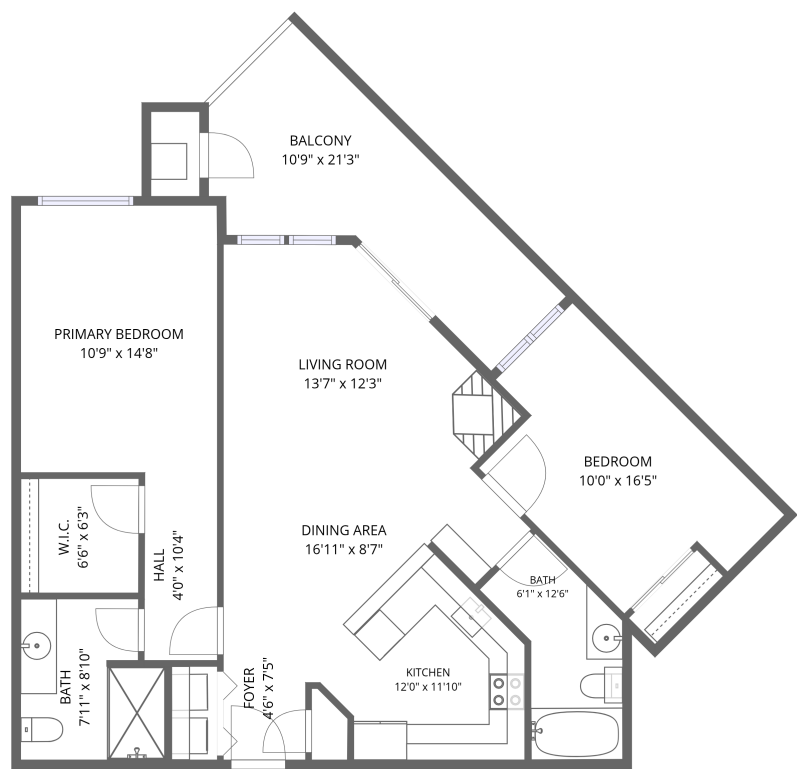
1st floor
