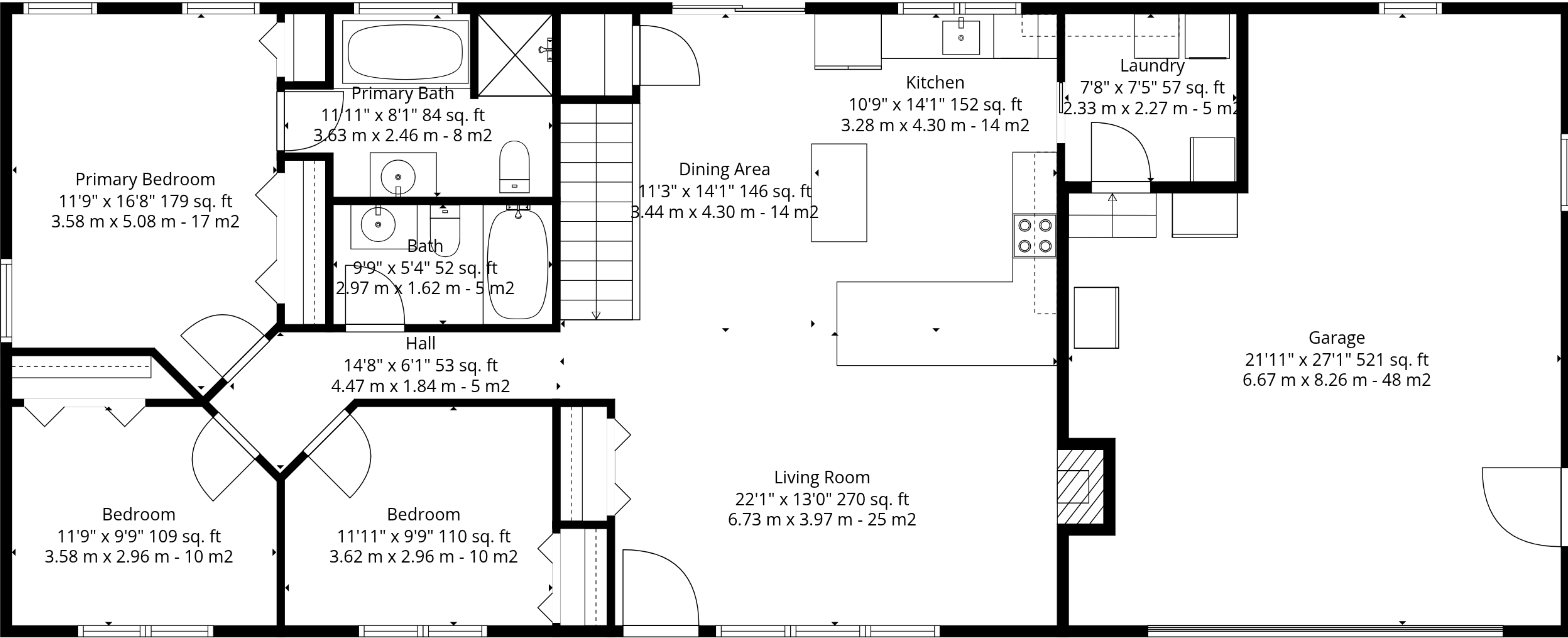
1st Floor
