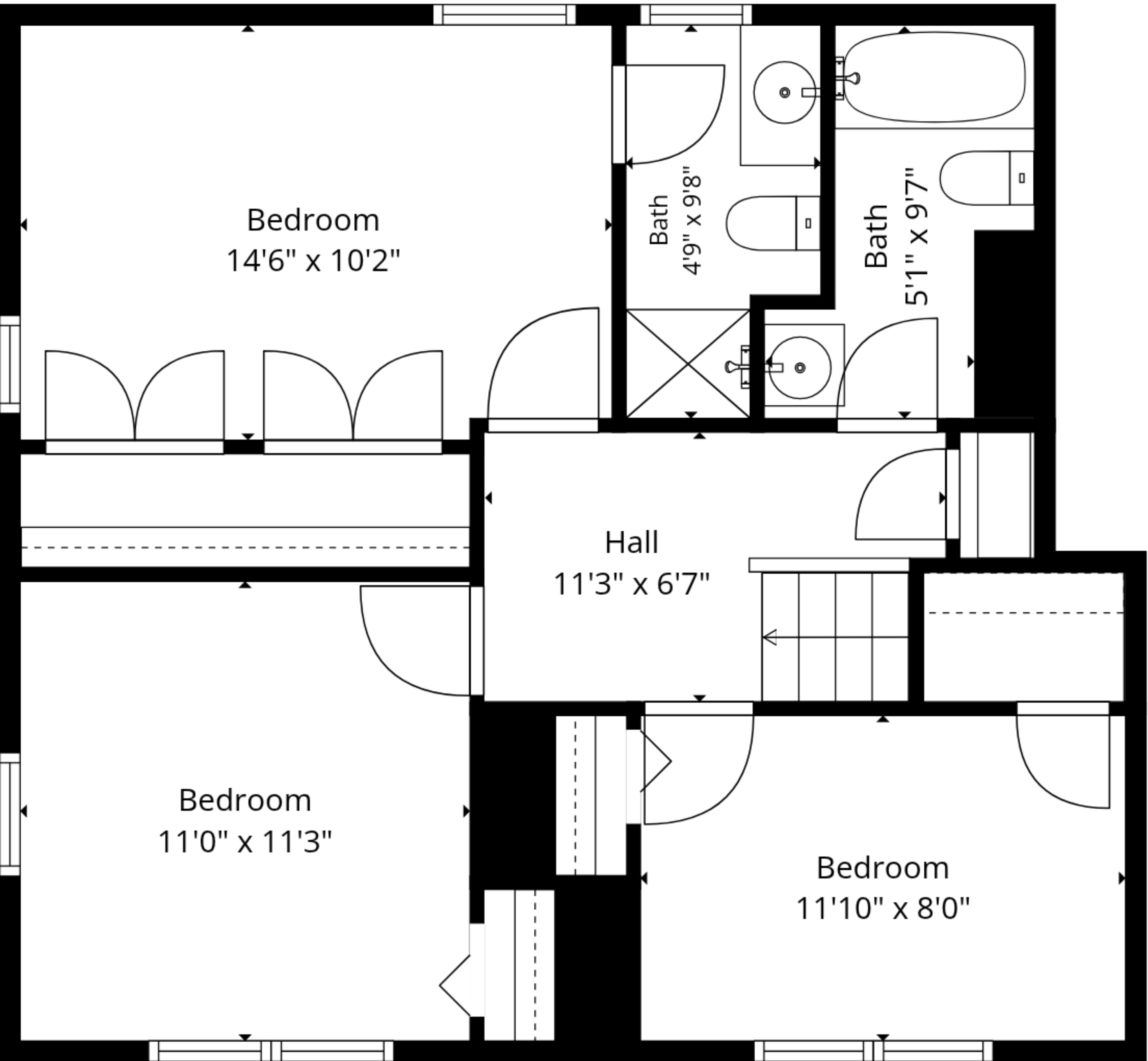
2nd Floor
