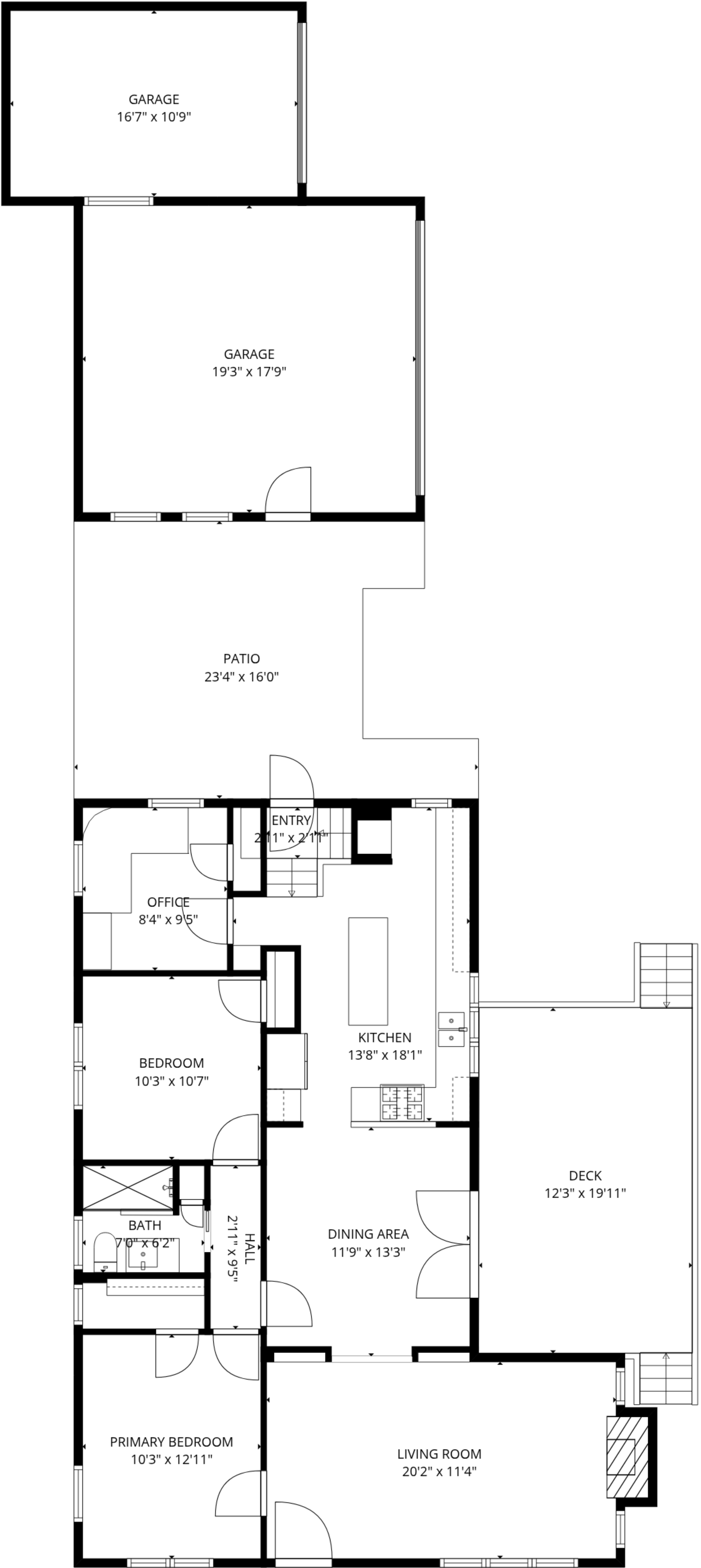
1st floor
