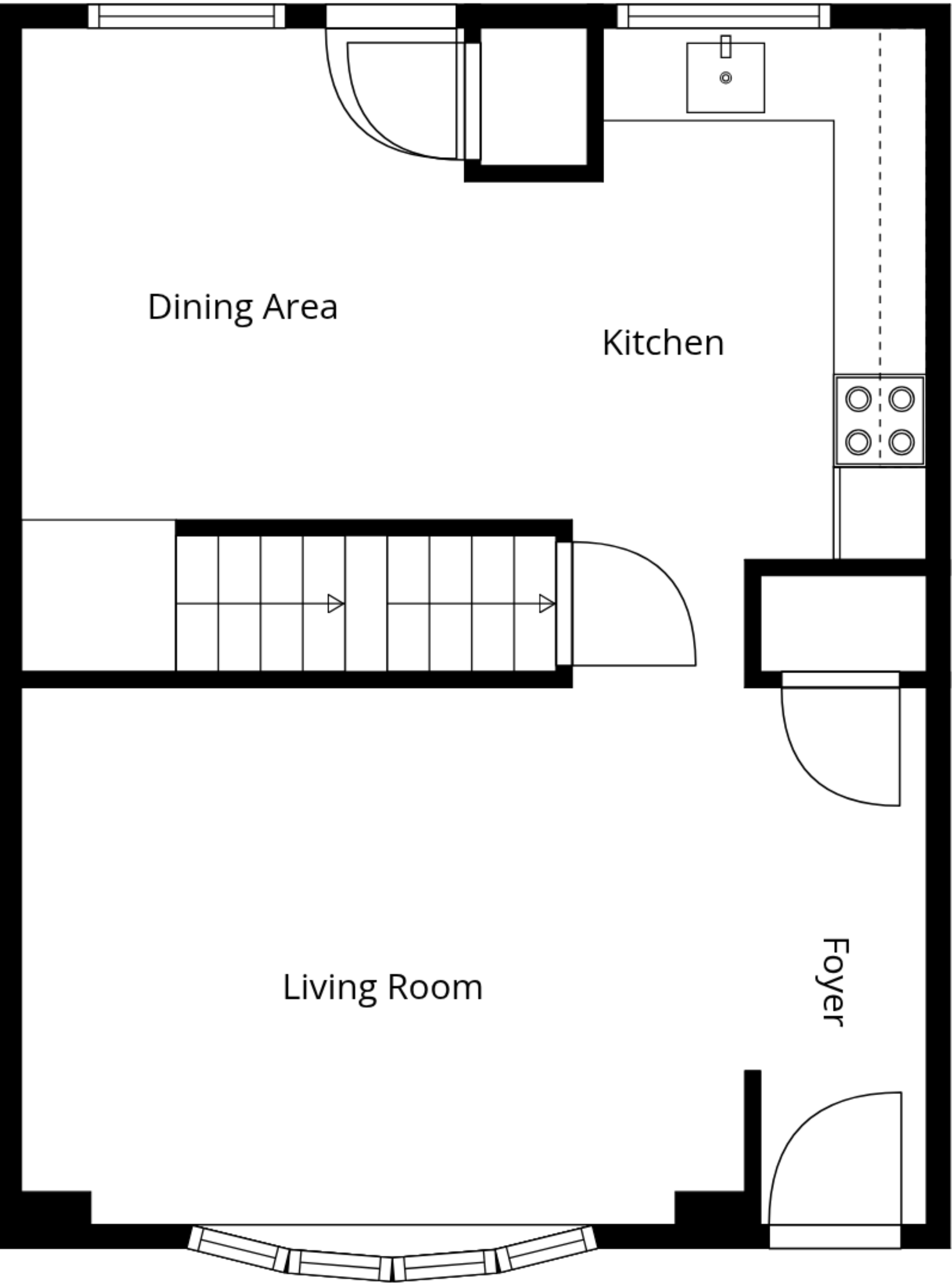
1st Floor
