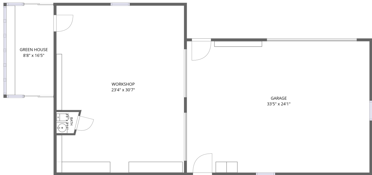
1st floor
