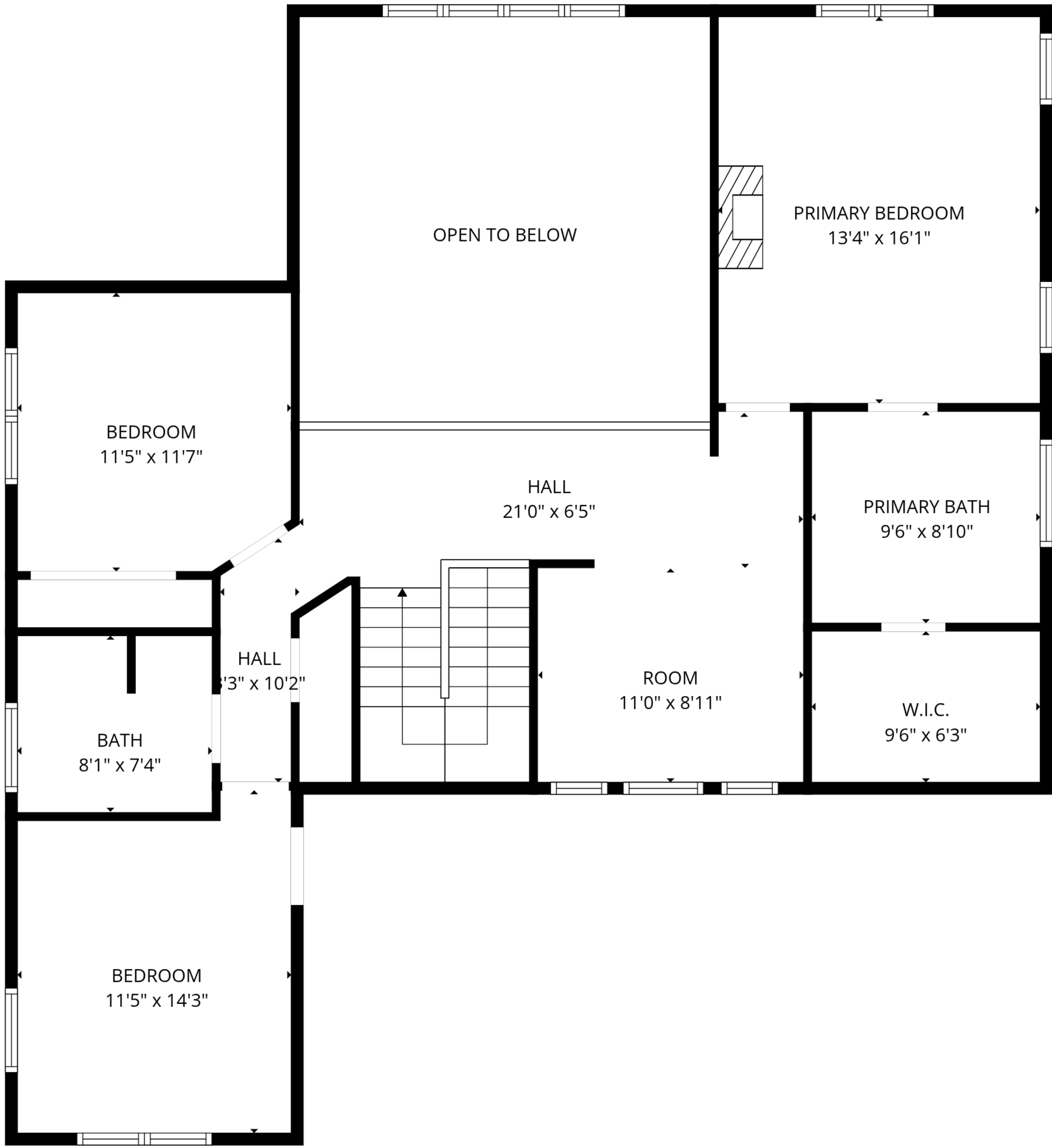
2nd floor
