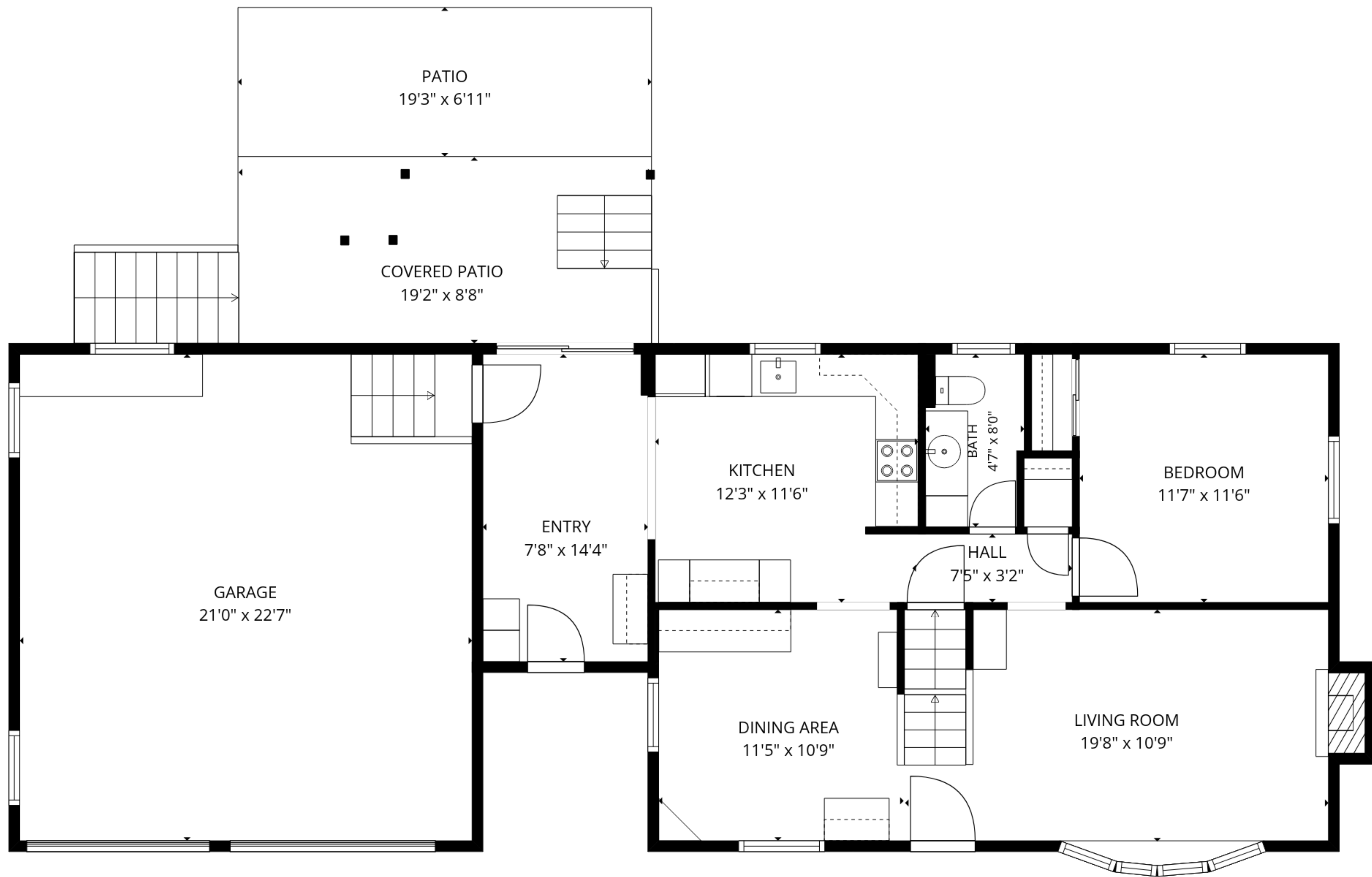
1st floor
