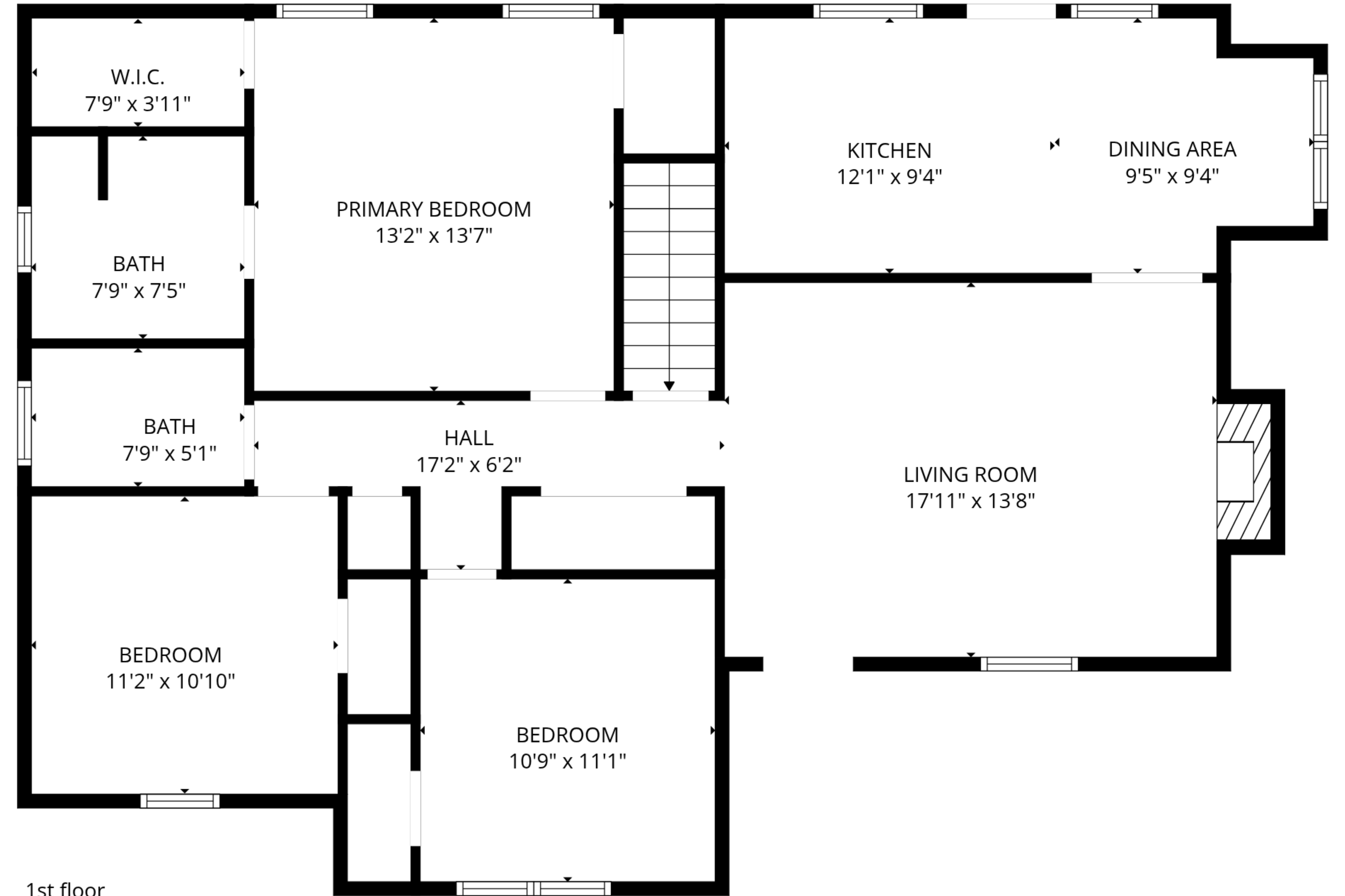
1st floor
