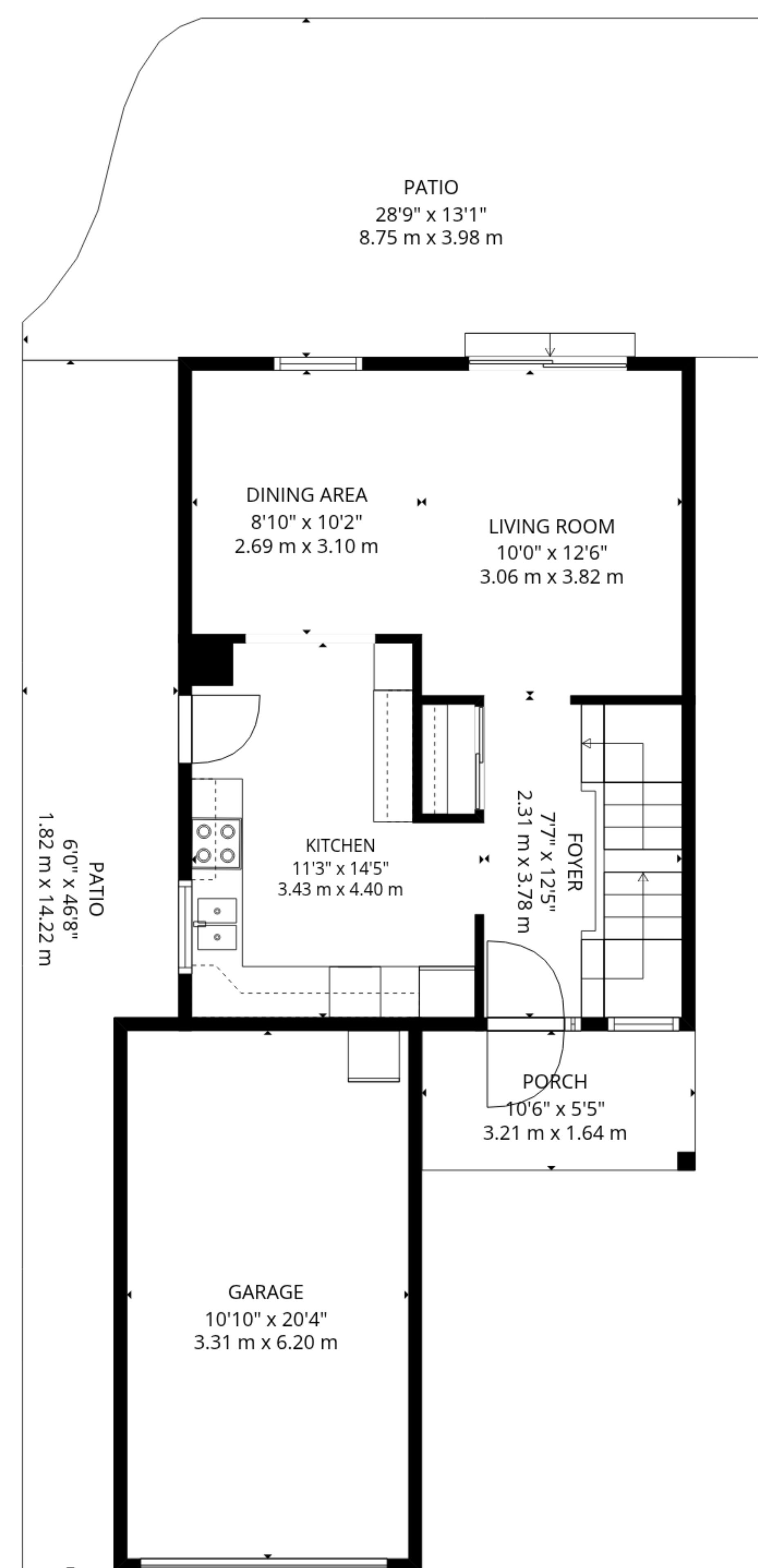
1ST FLOOR
