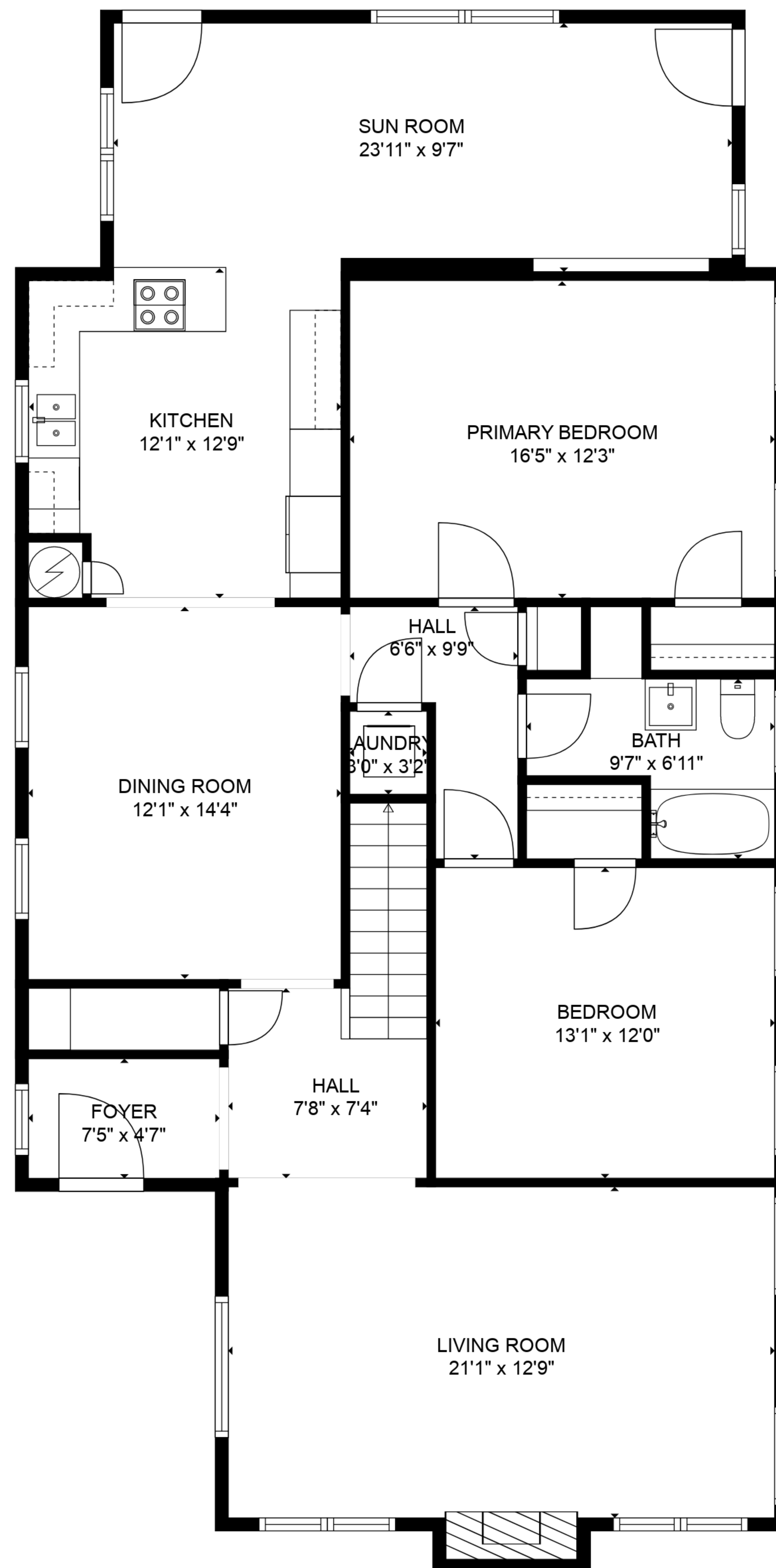
FLOOR 1
