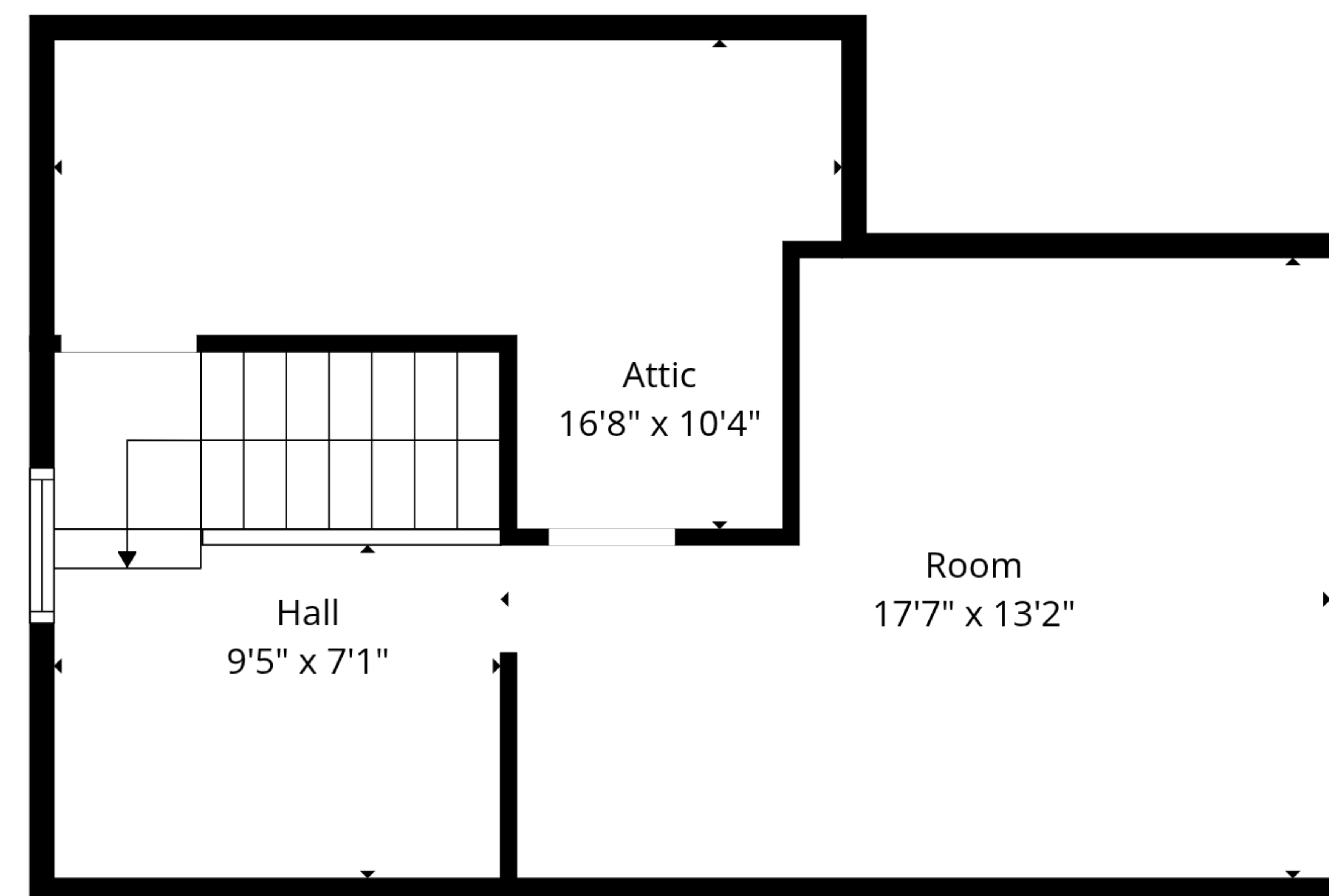
Floor 3
