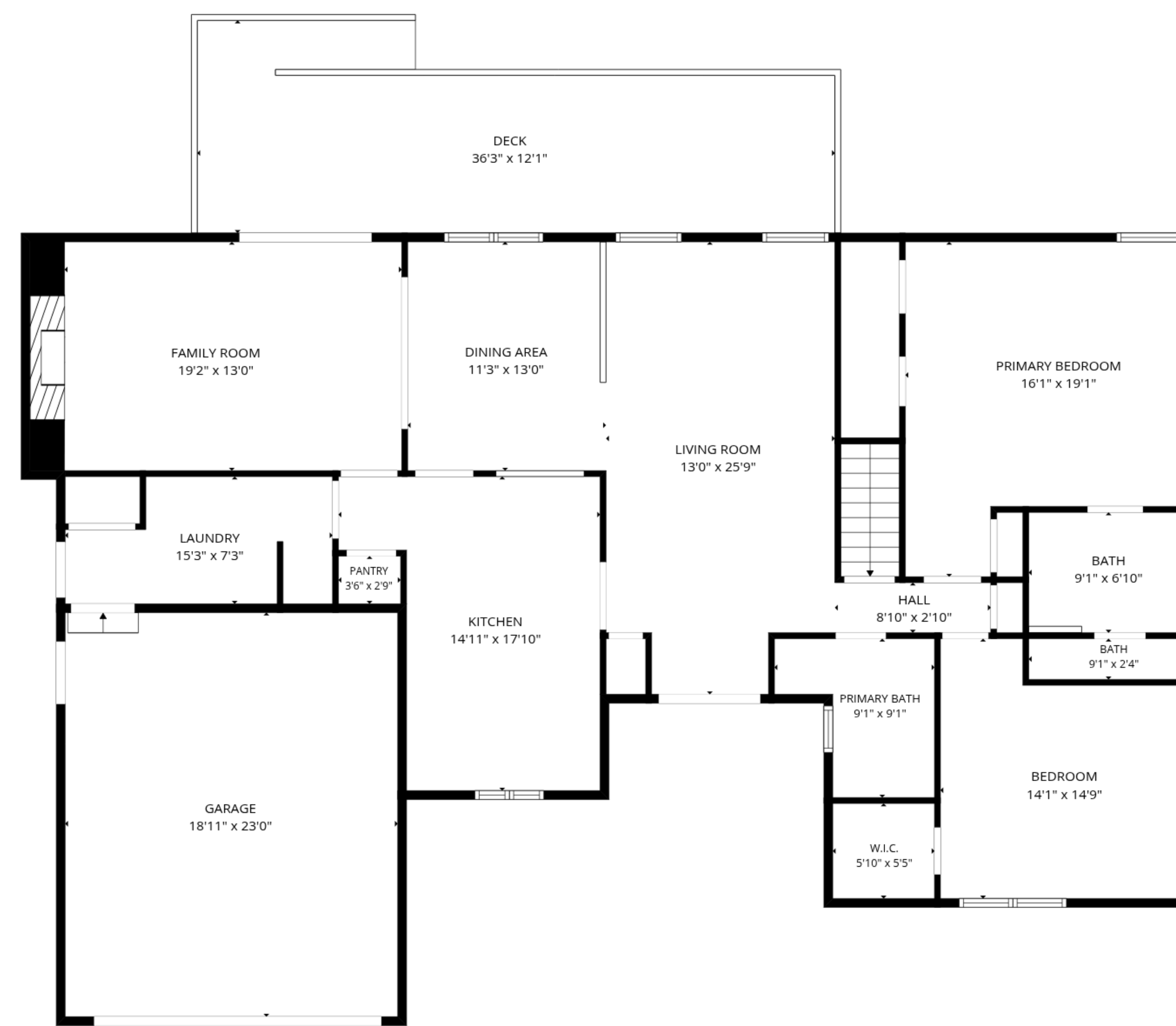
1st floor
