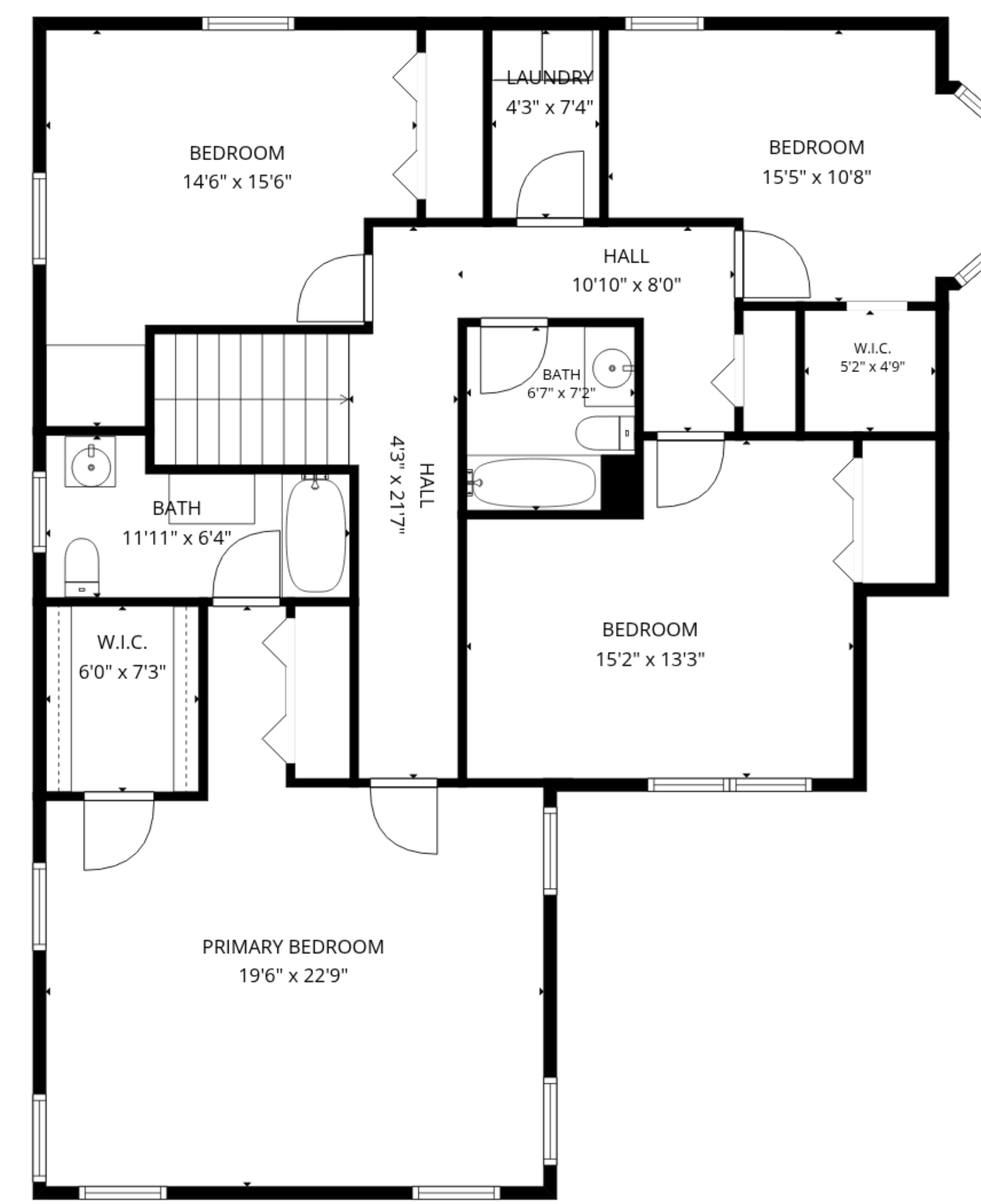
2nd floor
