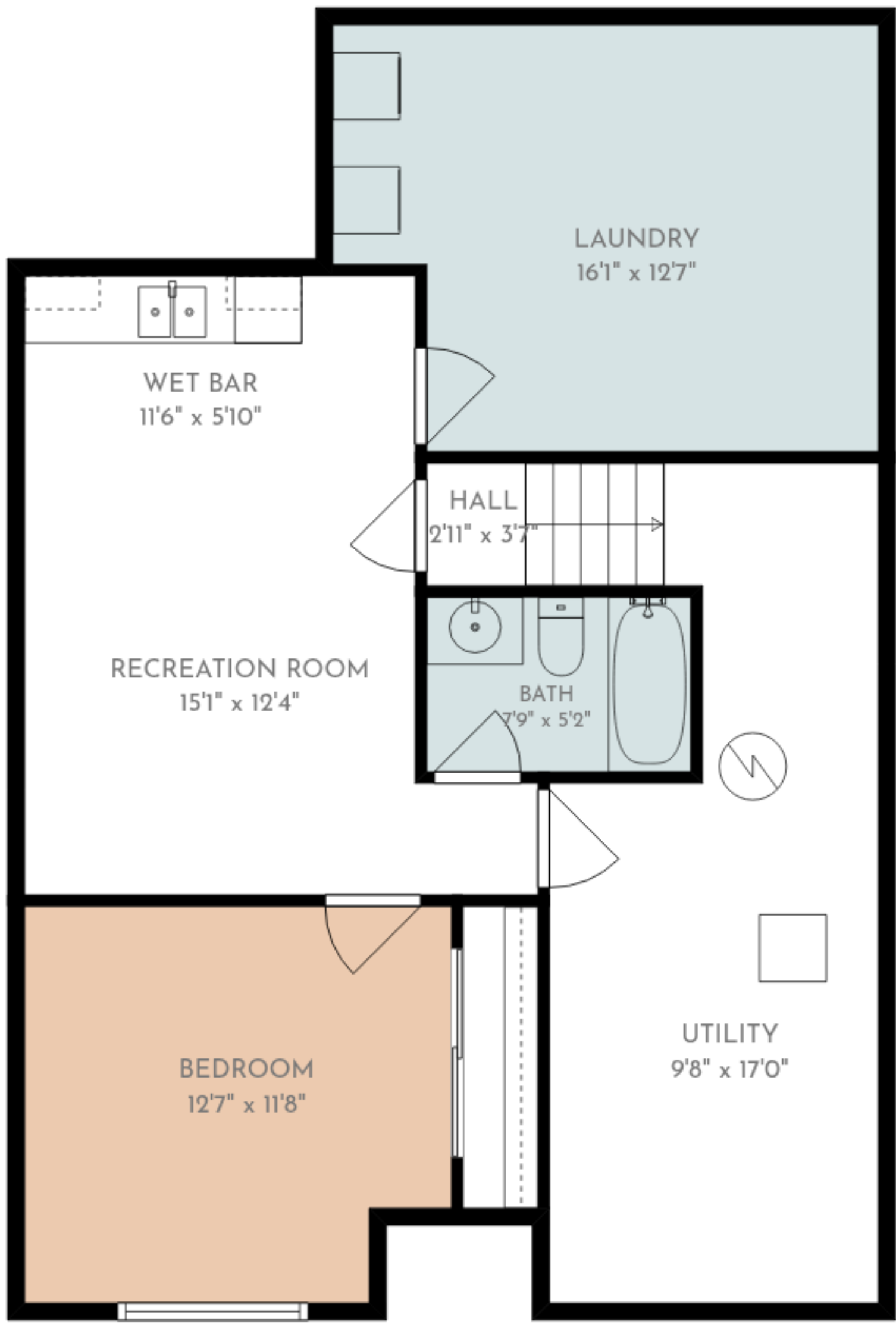
Basement
