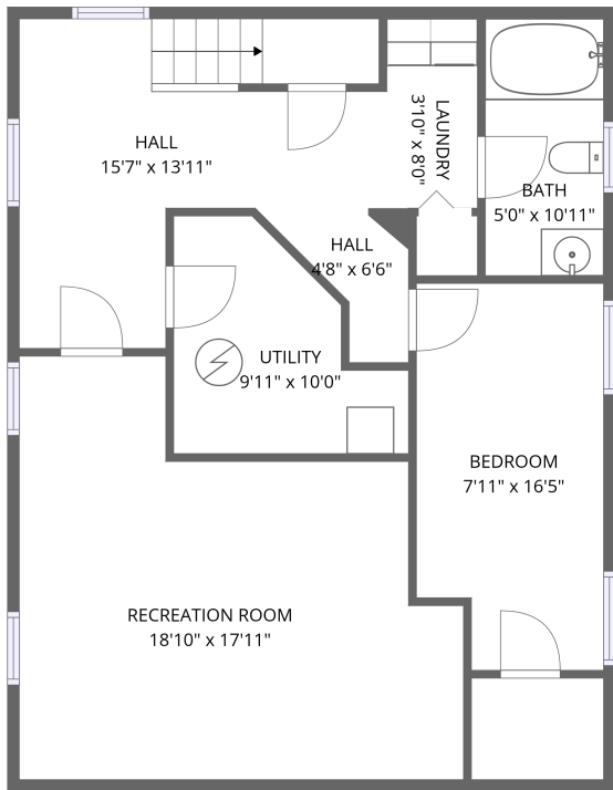
1st floor
