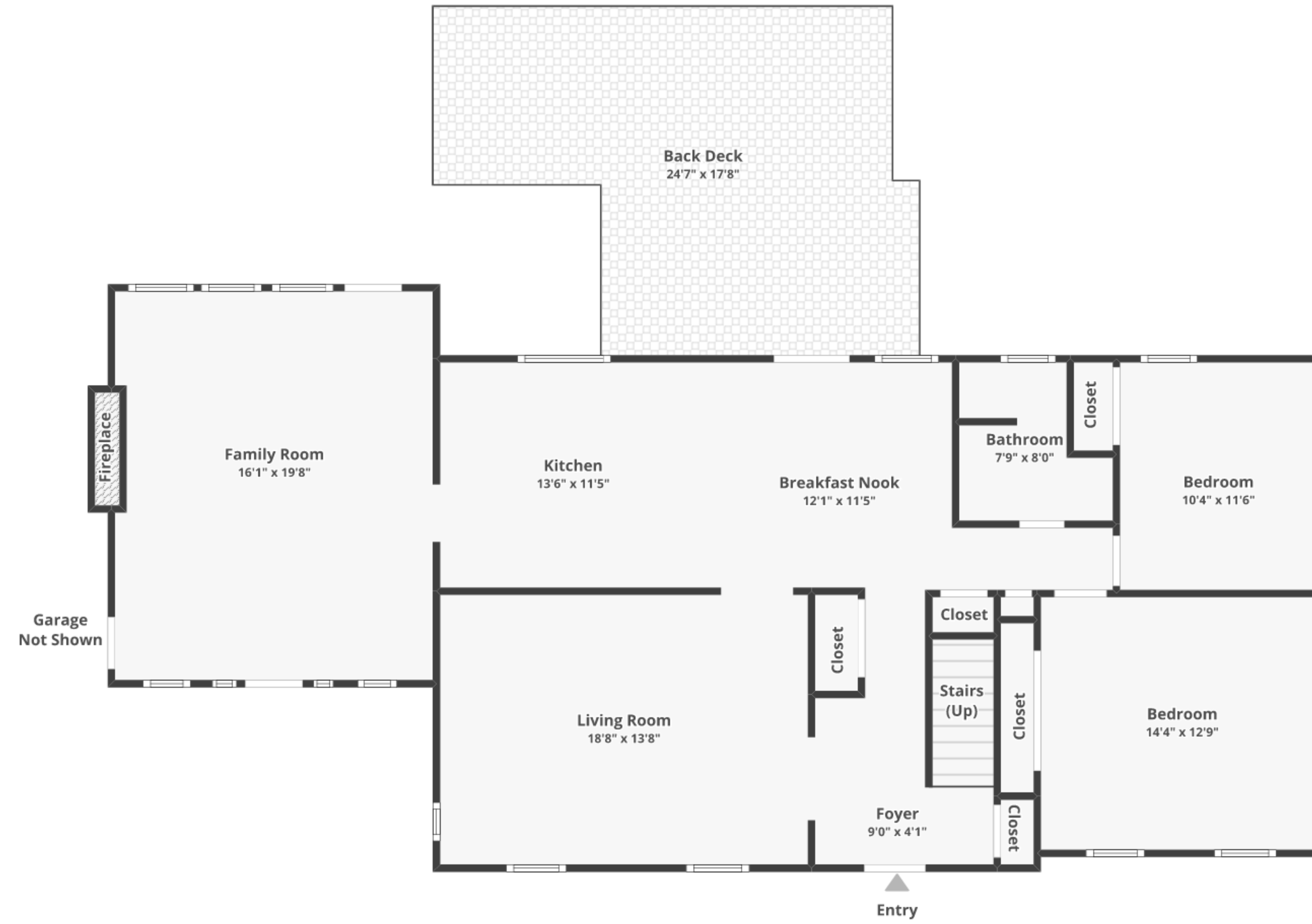
FLOOR 1 Finished area: ~1,375.99 sq. ft. Unfinished area: ~7.01 sq. ft.
