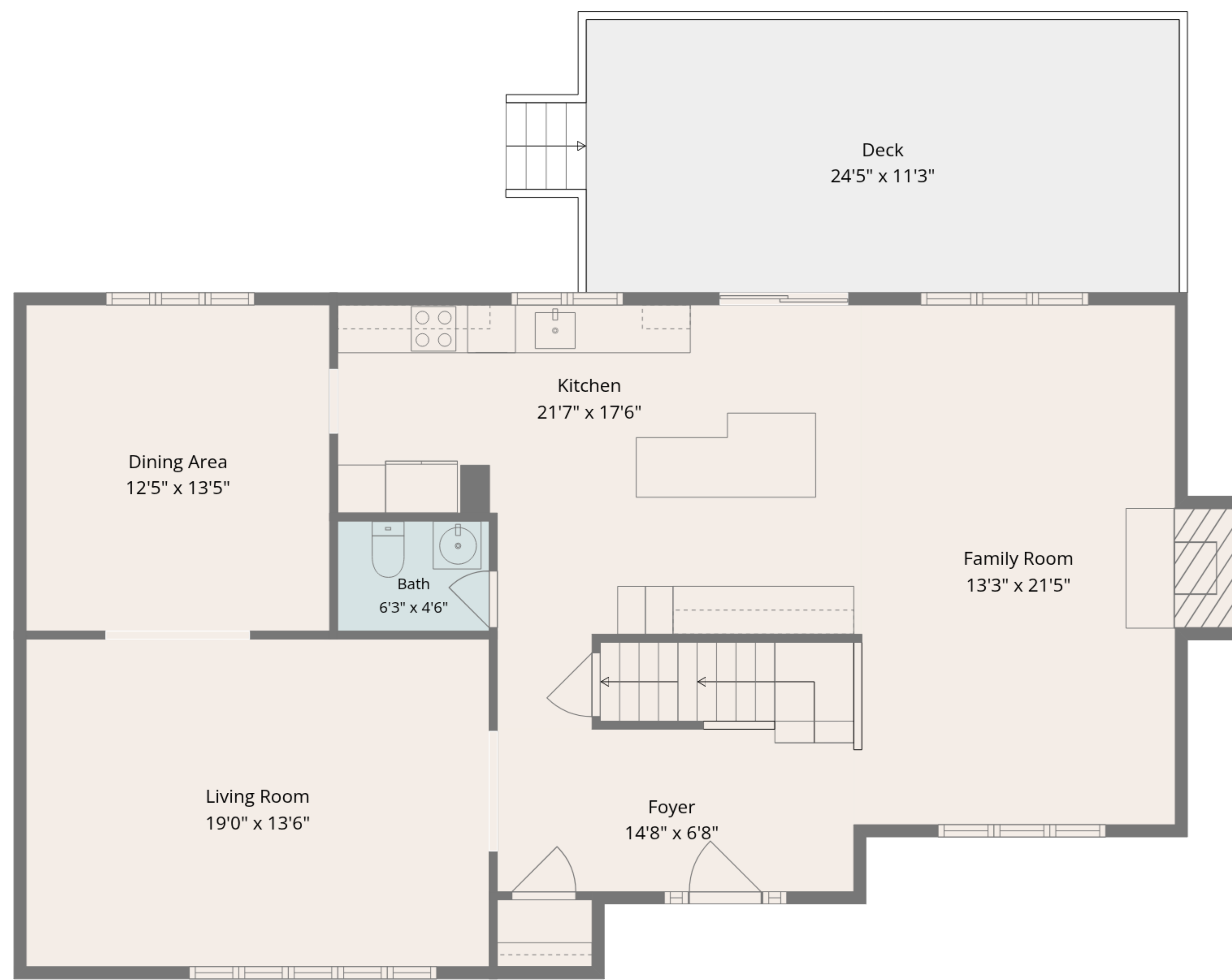
1st Floor
