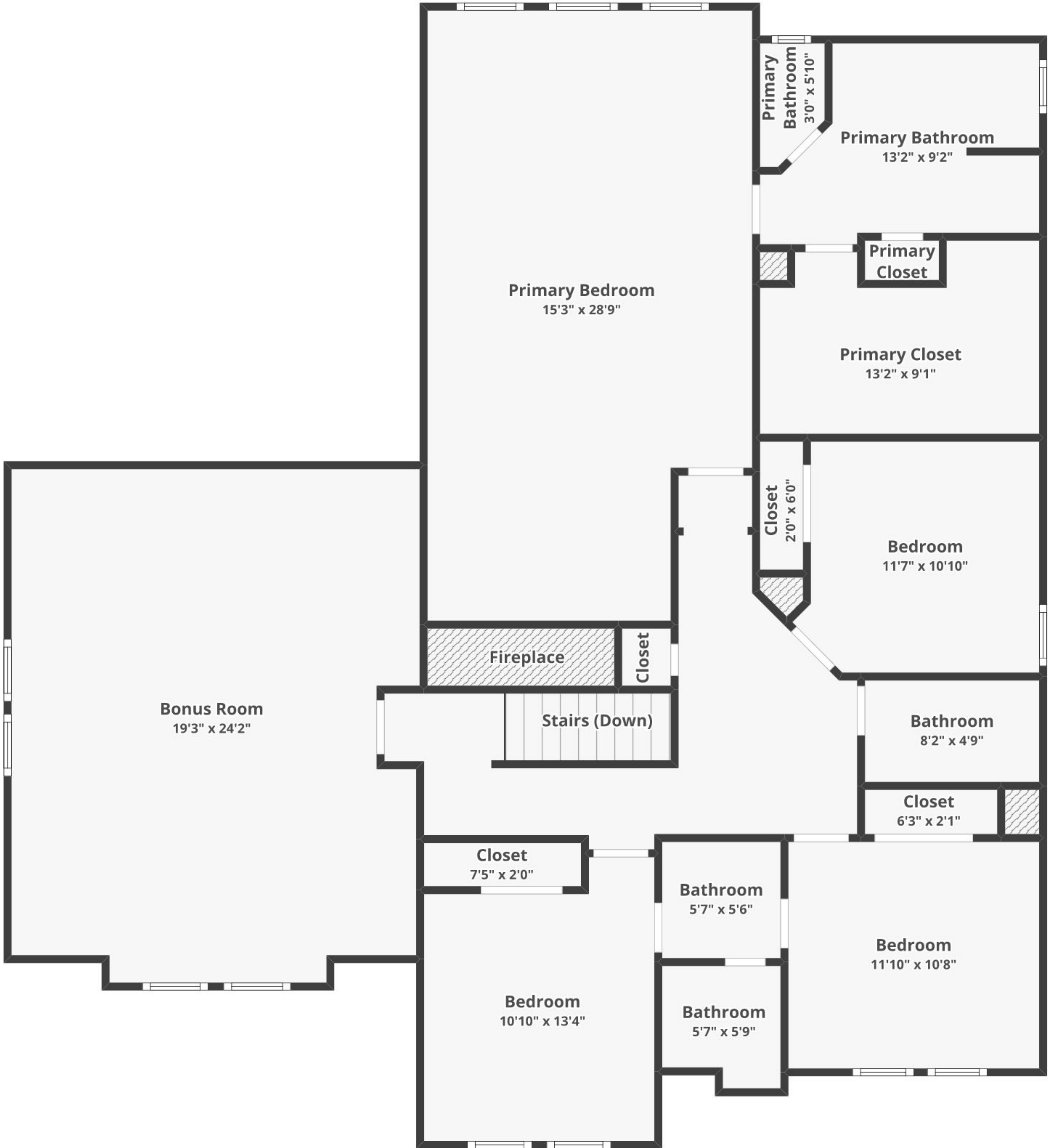
FLOOR 2
