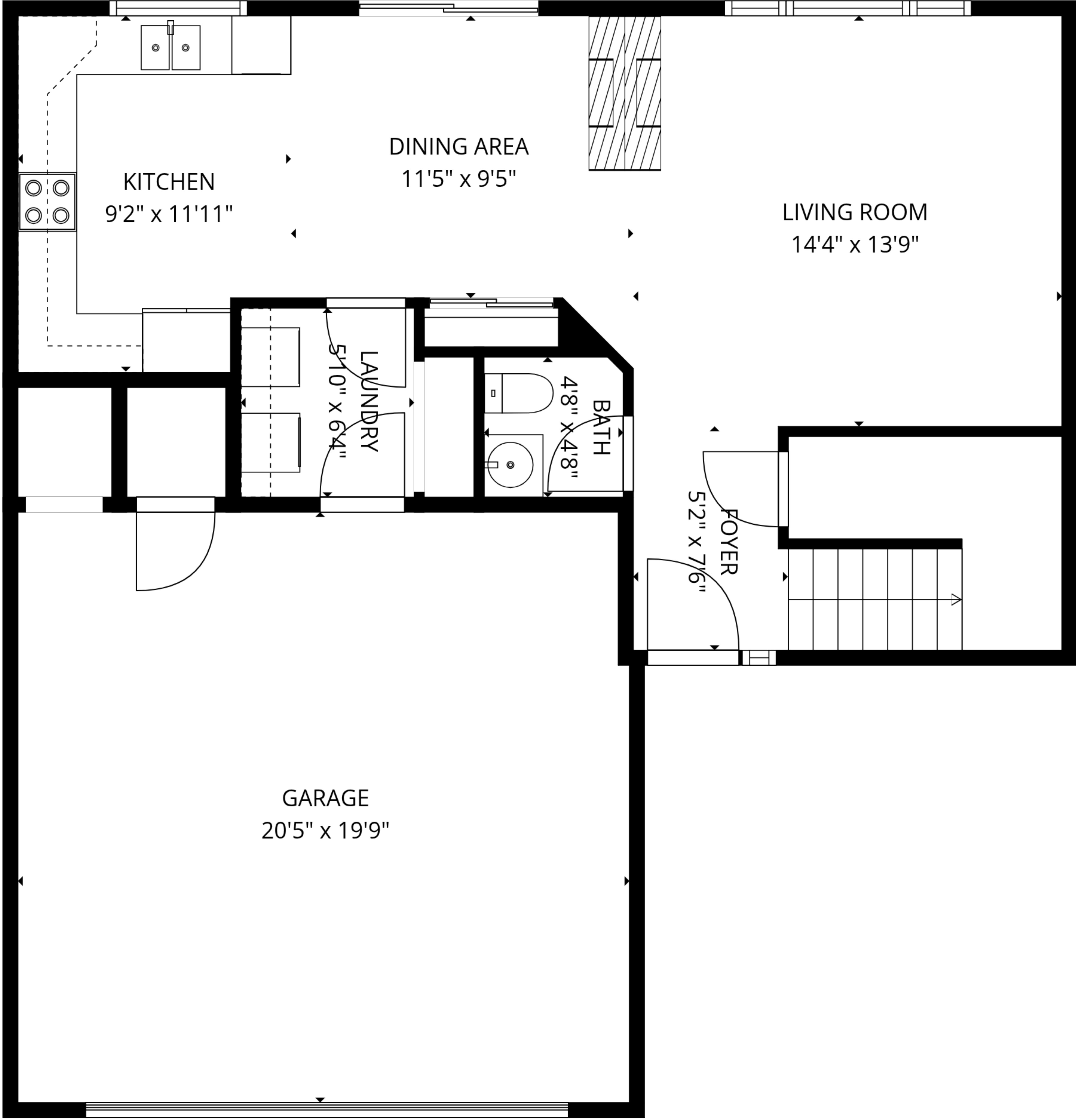
1st floor
